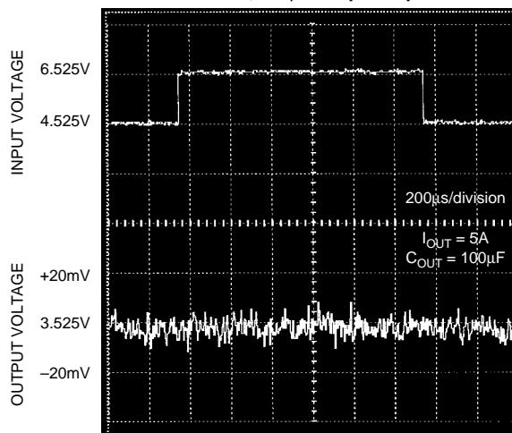
MIC29512 Line Transient Response with 5A Load, 100 \mu F Output Capacitance
