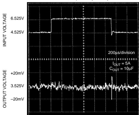
MIC29512 Line Transient Response with 5A Load, 10 \mu F Output Capacitance
