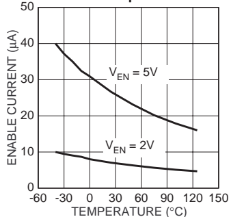
MIC29512 Enable Current vs. Temperature
