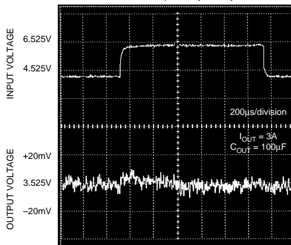
MIC29312 Line Transient Response with 3A Load, 100μF Output Capacitance
