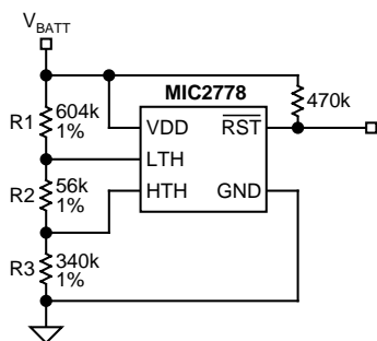
Figure 1. Example Circuit
