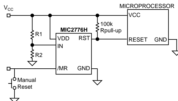
Figure 5. MIC2776H Valid Reset Below 1.2V
