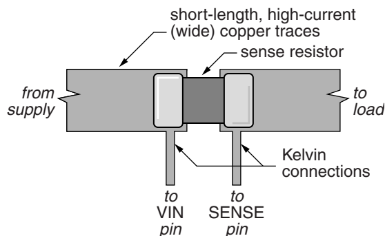
Figure 8. Layout Recommendation
