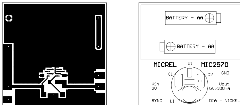
Component Side and Silk Screen (Not Actual Size)
