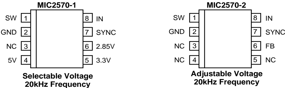
8-Lead SOIC (M)
