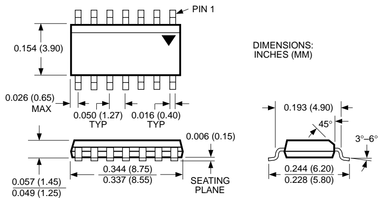
14-Pin Narrow SOP (M)
