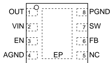
8-Pin MLF™ (BML) (Top View)
