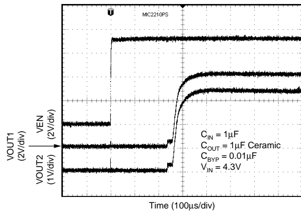
Enable Characteristics
