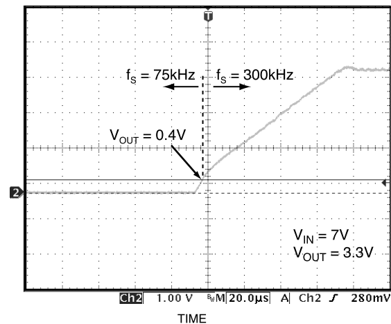
Figure 4. Startup Waveform
