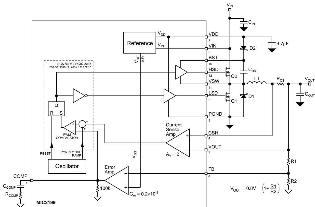
Figure 2. PWM Operation
