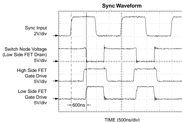
Figure 8. Sync Waveforms
