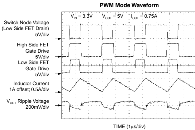
Figure 5 - PWM mode waveforms
