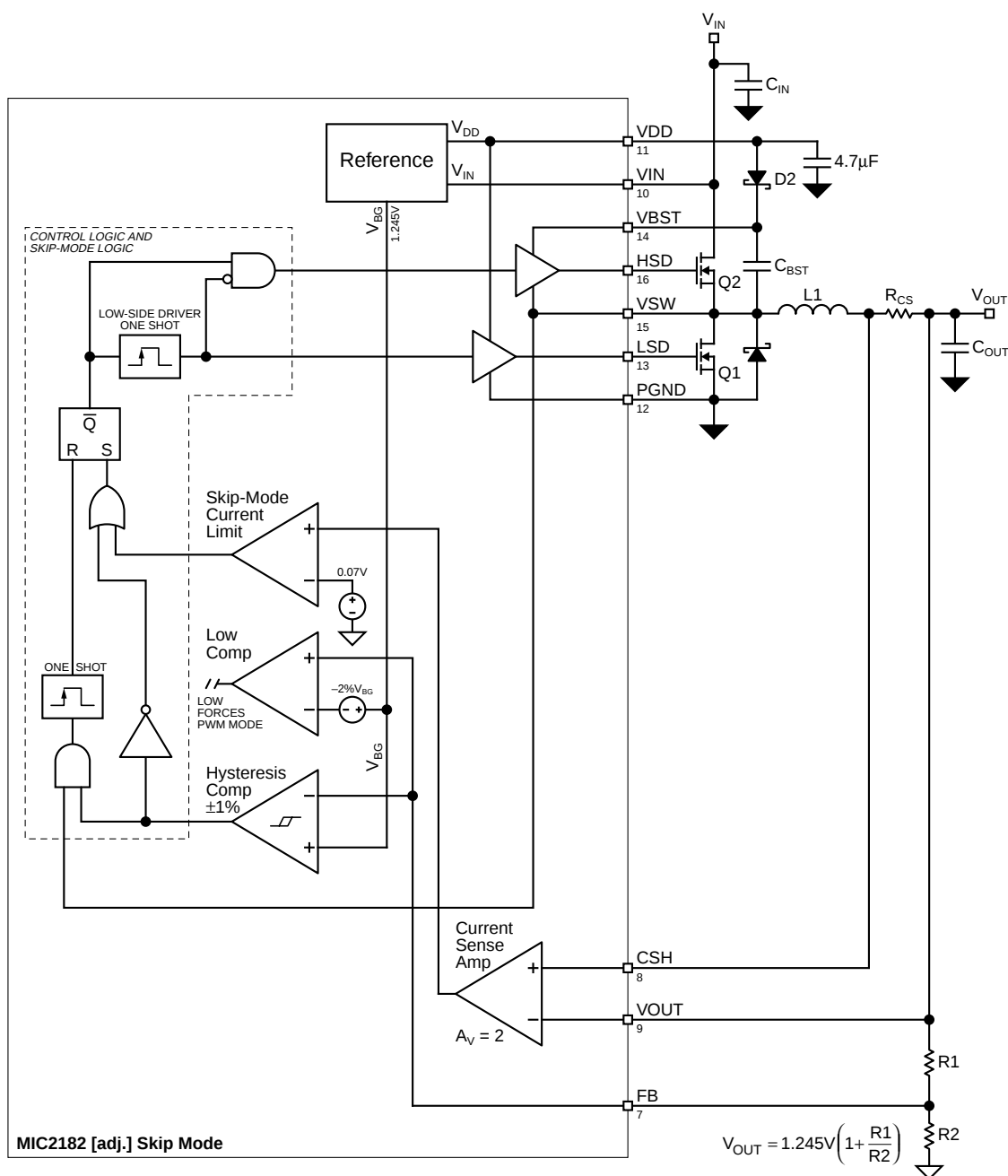
Figure 4. Skip-Mode Operation
