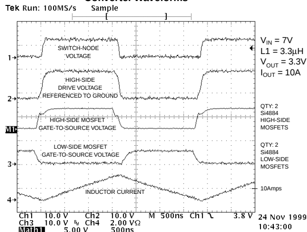
Converter Waveforms
