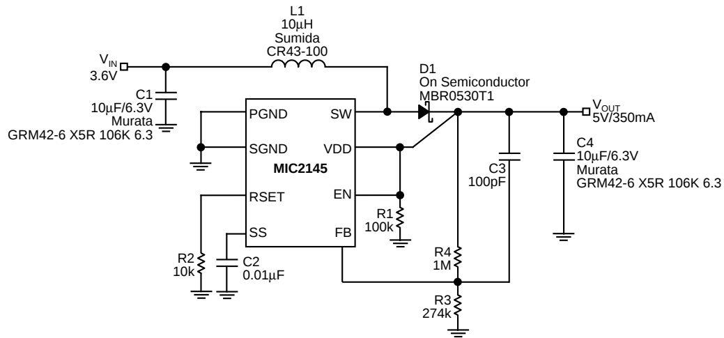
Figure 7. Bootstrap Configuration
