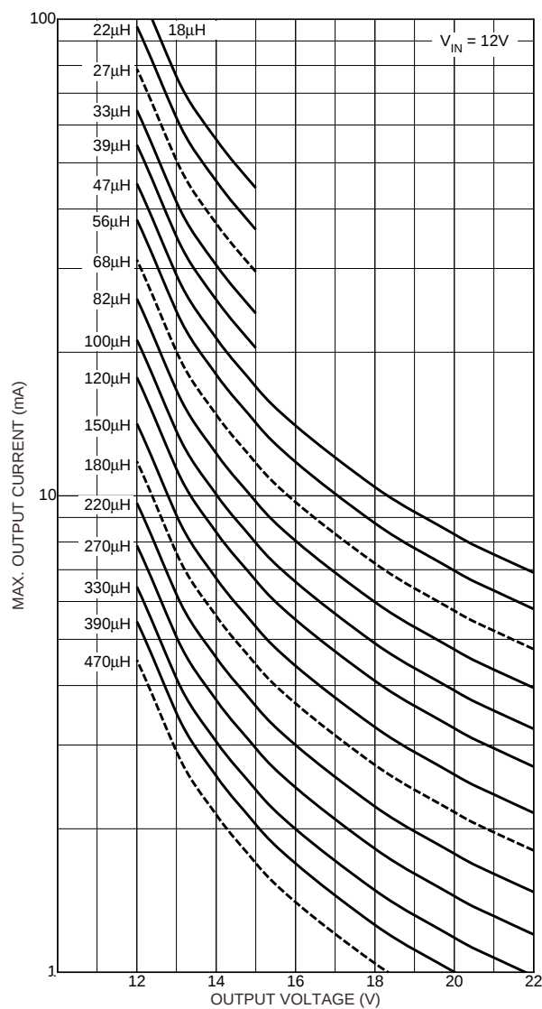
Figure 9. Inductor Selection for V_{IN} = 12V
