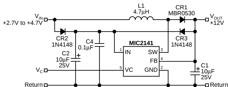
Figure 3. Bootstrap Configuration
