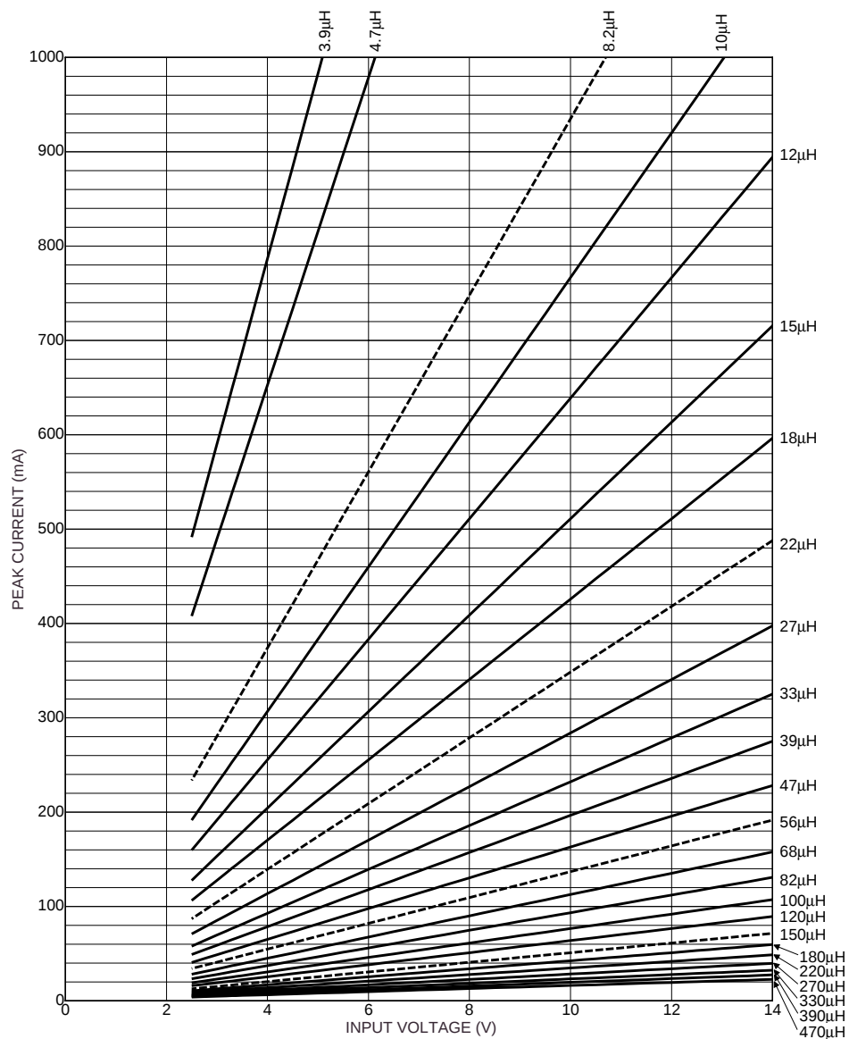
Figure 10. Peak Inductor Current vs. Input Voltage
