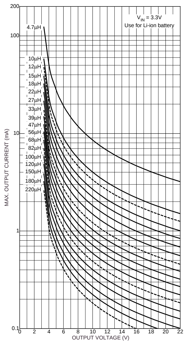
Figure 6. Inductor Selection for V_{IN} = 3.3V
