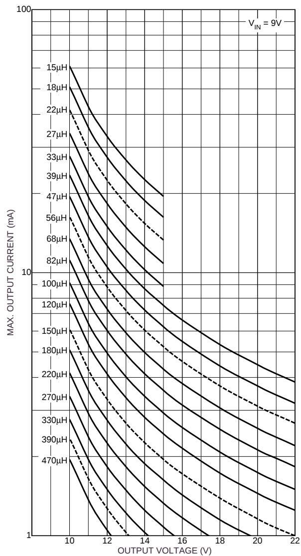
Figure 8. Inductor Selection for V_{IN} = 9V
