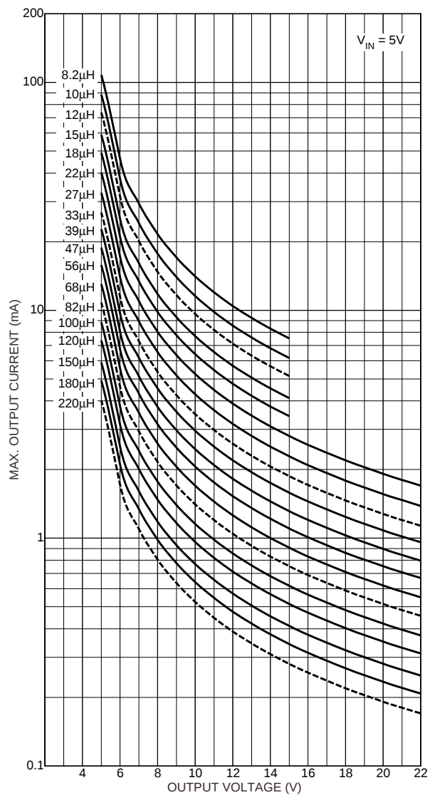
Figure 7. Inductor Selection for V_{IN} = 5V
