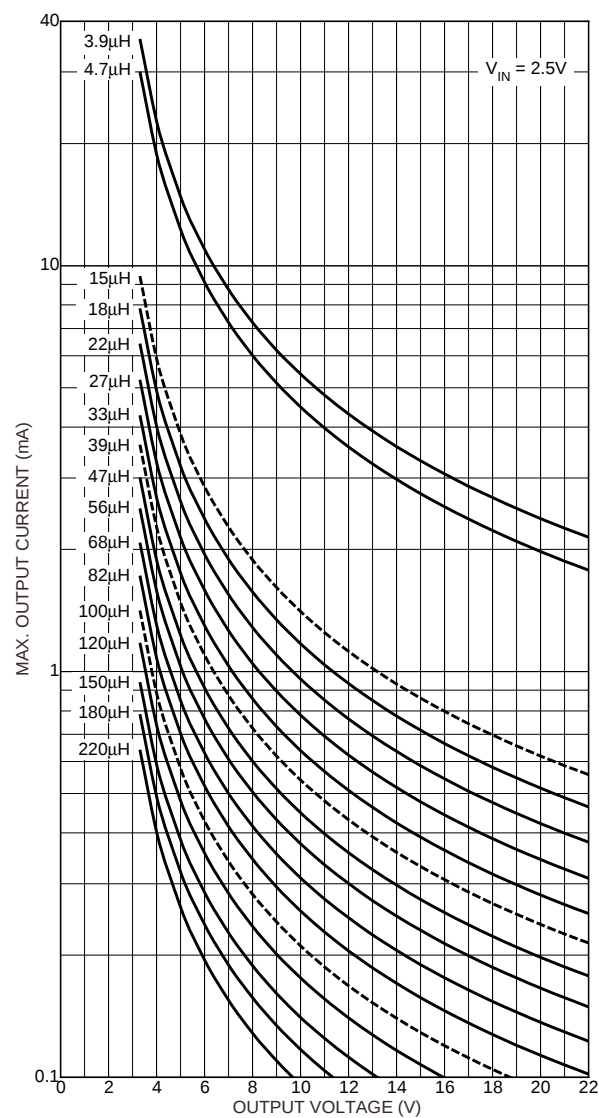
Figure 5. Inductor Selection for V_{IN} = 2.5V
