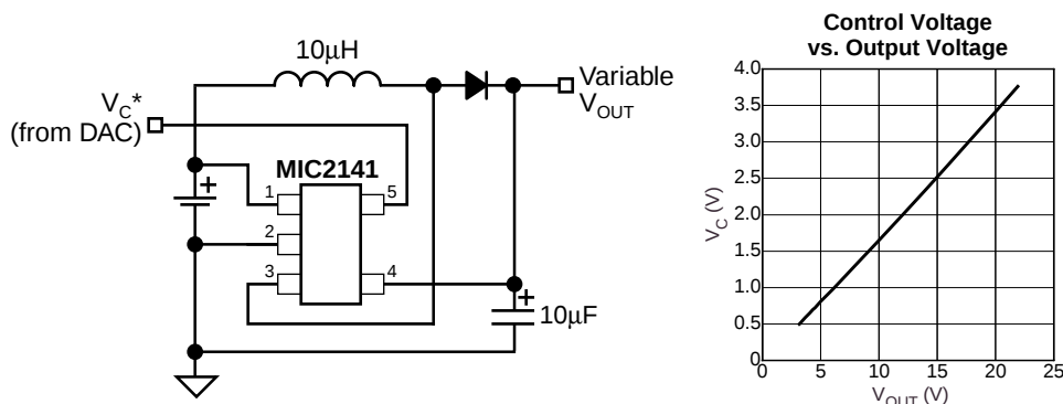
DAC-Controlled LCD Bias Voltage Supply
