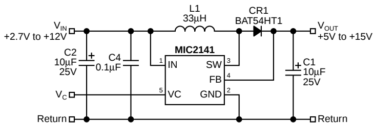
Figure 1. Basic Configuration
