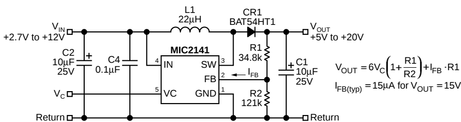
Figure 2. Gain-Boost Configuration
