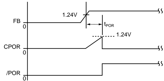
Figure 2. Power-On Reset Response
