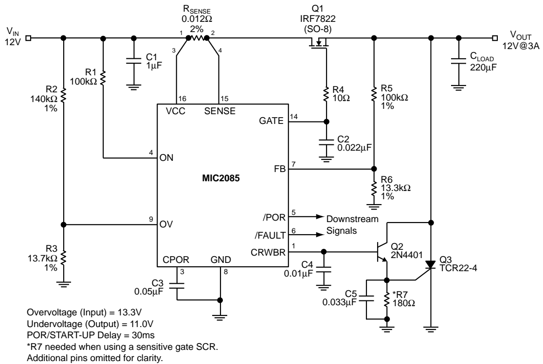
Figure 5. Undervoltage/Overvoltage Circuit
