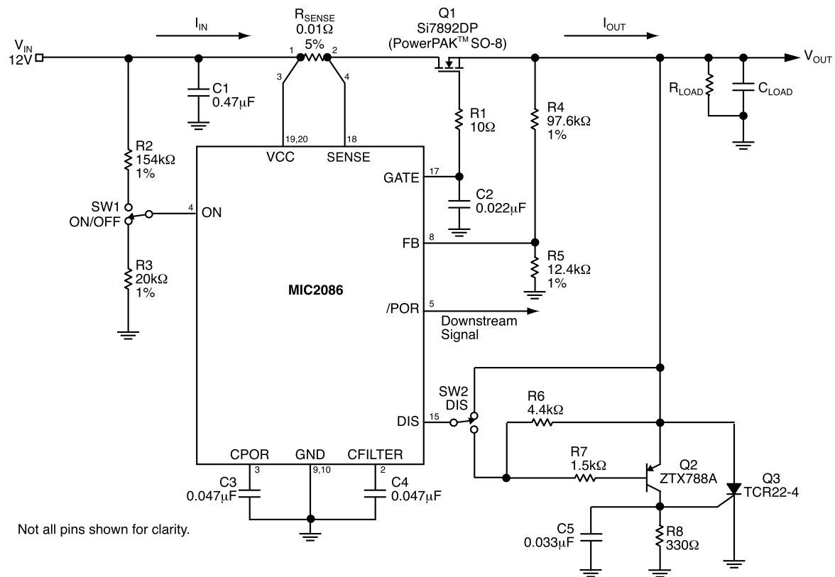
Test Circuit
