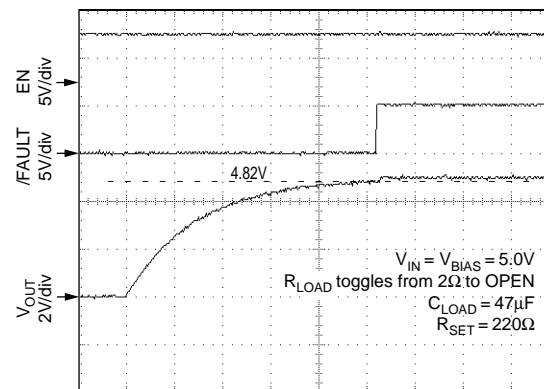
Latched Output Reset MIC2045
