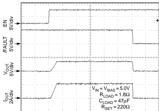
Latched Output MIC2045
