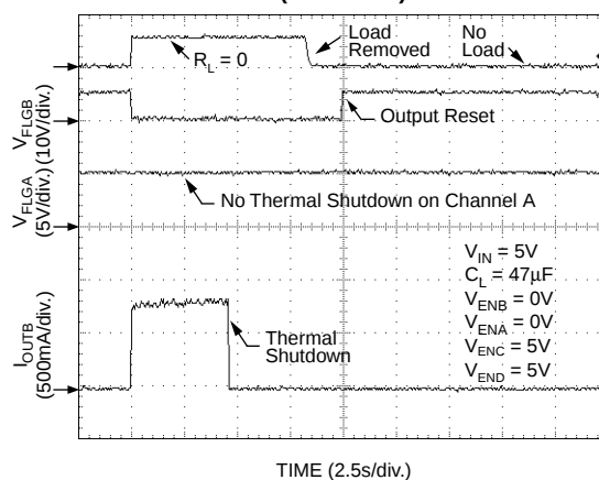
Independent Thermal Shutdown (MIC2077-2)
