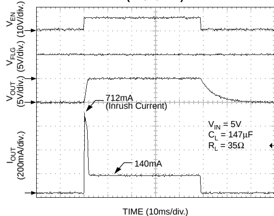
Turn-On/Turnoff (MIC2027-1)
