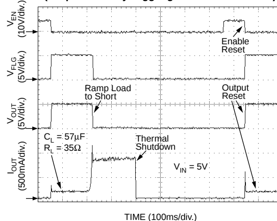
Thermal Shutdown (Output Reset by Toggling Enable—MIC2077-2)
