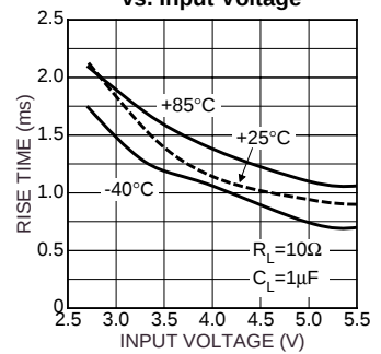
Turn-Off Rise Time vs. Input Voltage
