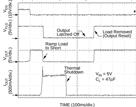
Thermal Shutdown (Output Reset by Removing Load—MIC2077-2)
