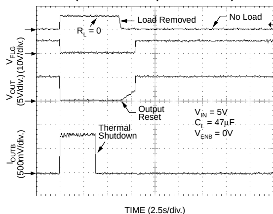
Thermal Shutdown (MIC2077-2—Output Latched Off)
