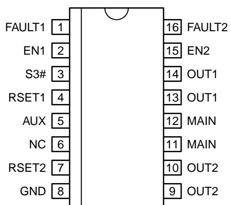
16-Pin QSOP (QS)
