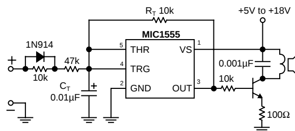
Figure 9. Audible Voltmeter
