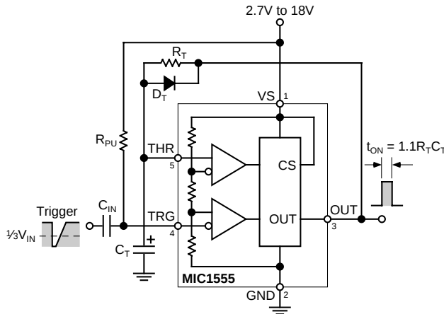
Figure 1. One-Shot Diagram
