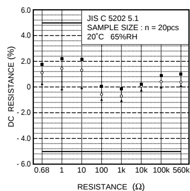
Fig.5 DC resistance
