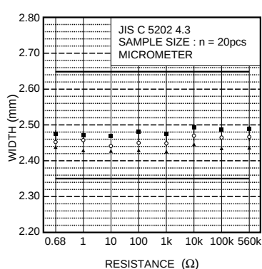
Fig.3 Dimensions (width)
