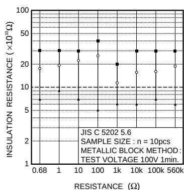
Fig.8 Insulation resistance
