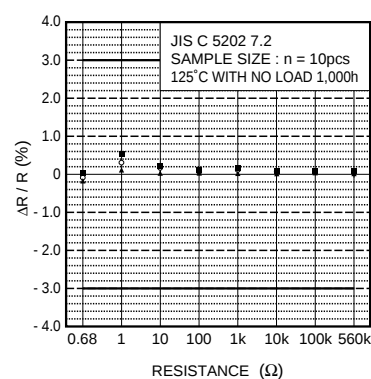
Fig.13 Resistance to dry heat
