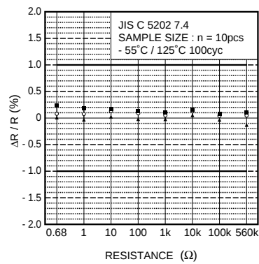
Fig.17 Temperature cycling
