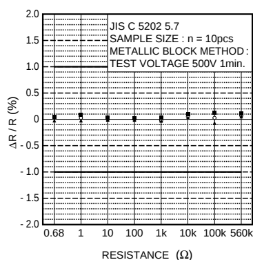
Fig.9 Withstand voltage
