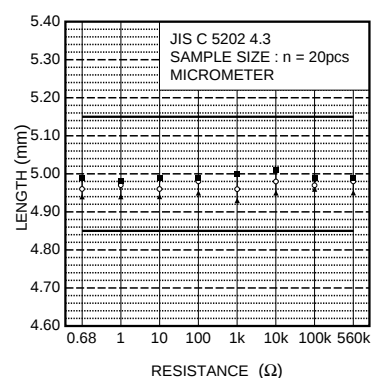
Fig.2 Dimensions (length)
