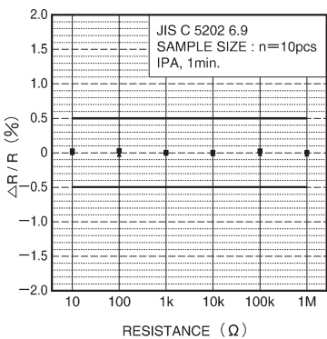
Fig.16 Resistance to solvents
