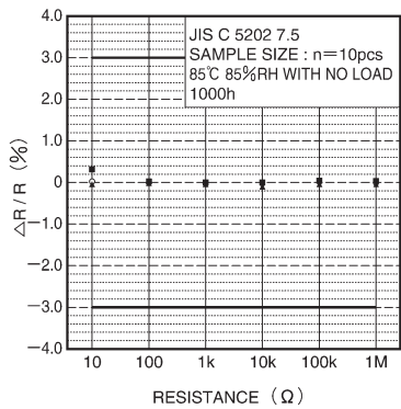
Fig.14 Humidity resistance (steady state)
