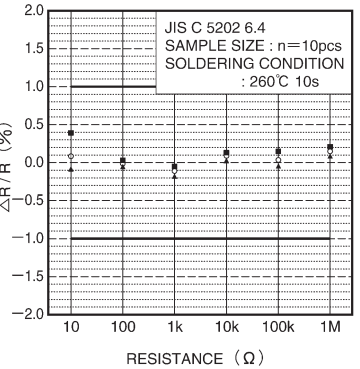
Fig.10 Resistance to soldering heat
