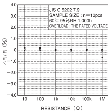
Fig.13 Endurance (under load in damp environment)
