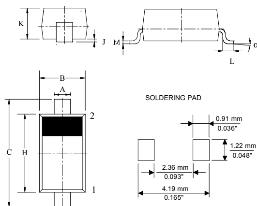
Outline SOD123
