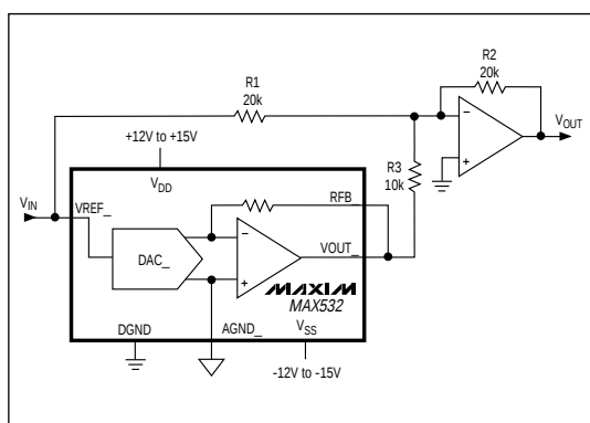
Figure 10. Bipolar Operation
