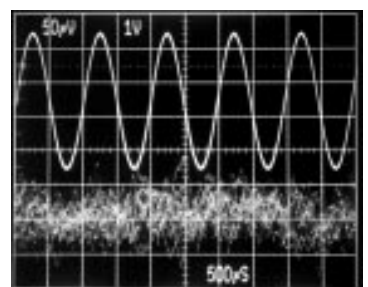
MAX517/MAX519 REFERENCE FEEDTHROUGH AT 1kHz
