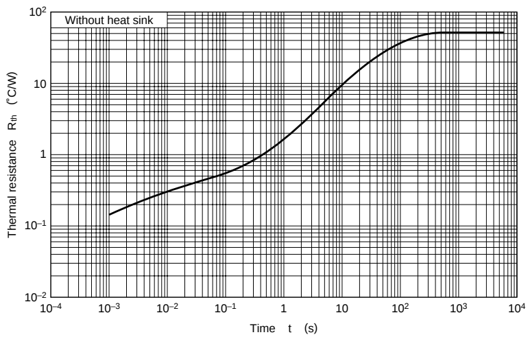
R_{th(t)} - t
