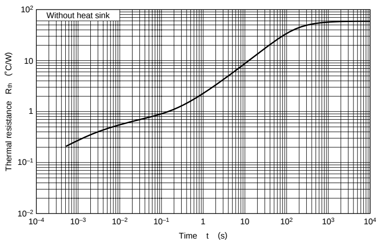
R_{th(t)} - t
