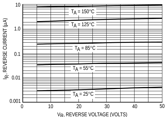
Figure 2. Reverse Current
