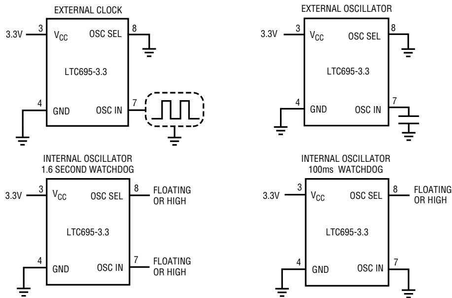
Figure 12. Oscillator Configurations
