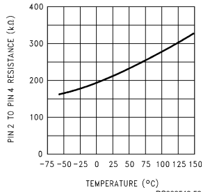
LP2951 Divider Resistance
