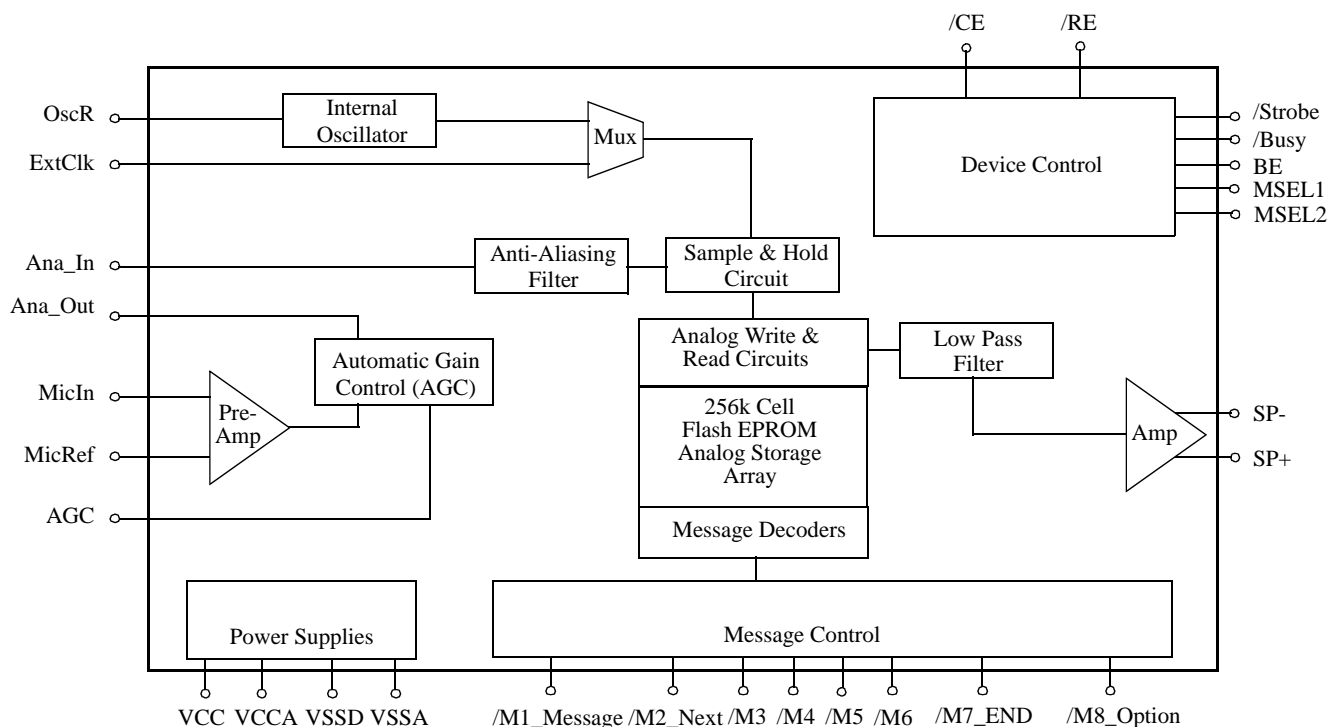
Figure 2 IVS1560 Block Diagram
