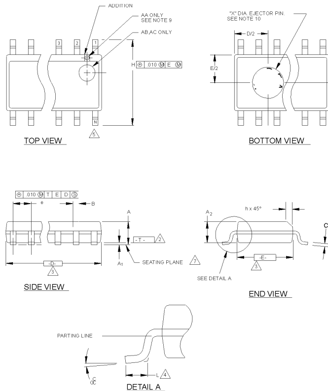
Figure 6 28-Pin Plastic Small-Outline Integrated Circuit (SOIC)
