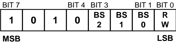
Figure 5. Device Addressing
