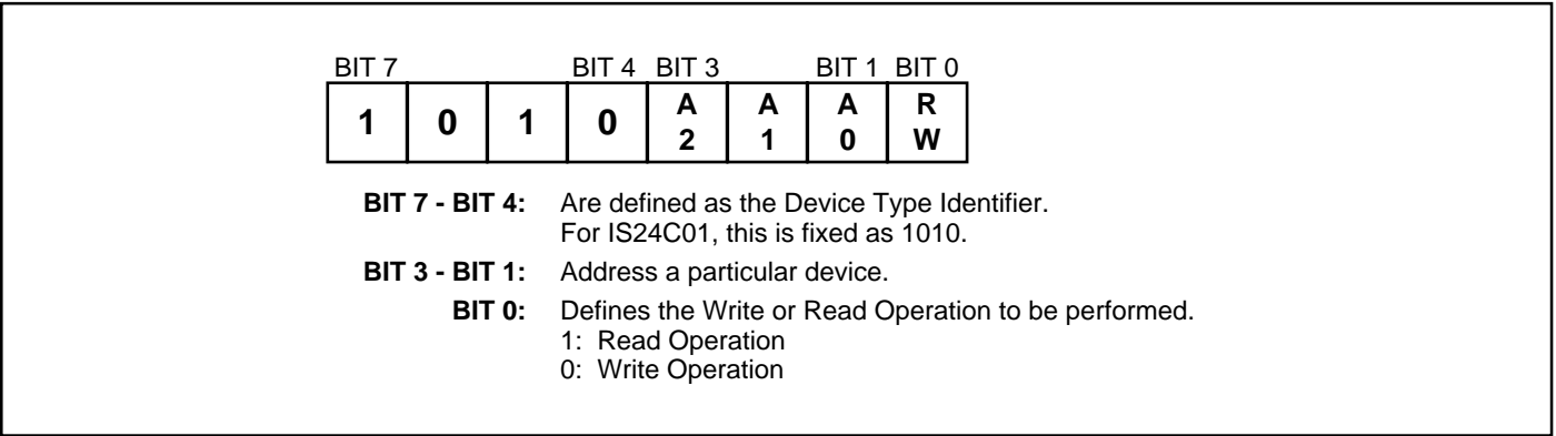
Figure 5. Device Addressing Byte Definitions
