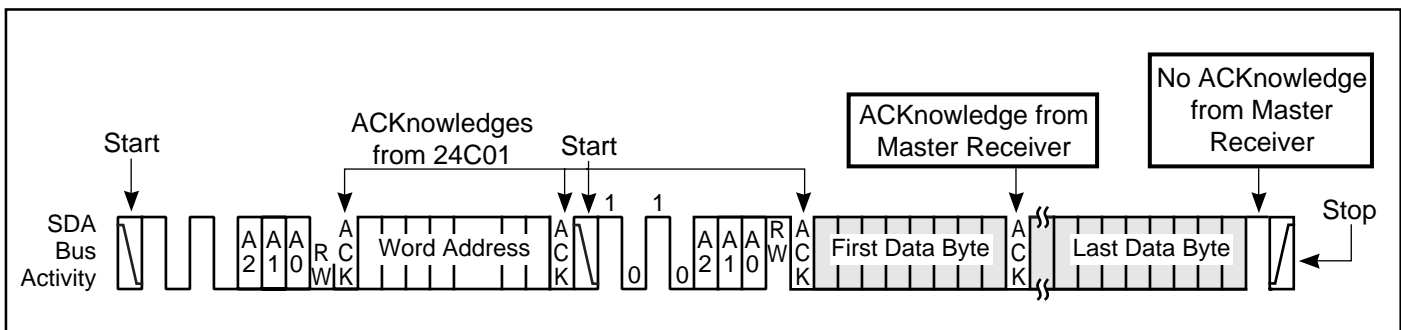
Figure 9. Sequential Read
