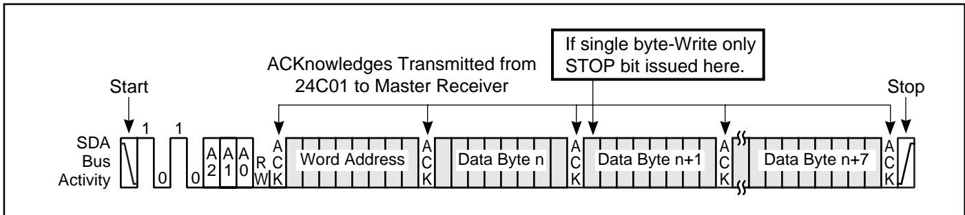
Figure 6. Write Operation
