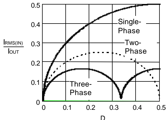
Figure 12 - Normalized input RMC current vs. duty cycle.
