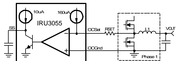
Figure 8 - Diagram of the over current sensing.
