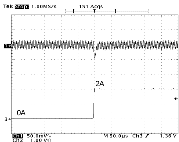
Figure 19 - Transient response @ I_{OUT}=0 to 2A.
