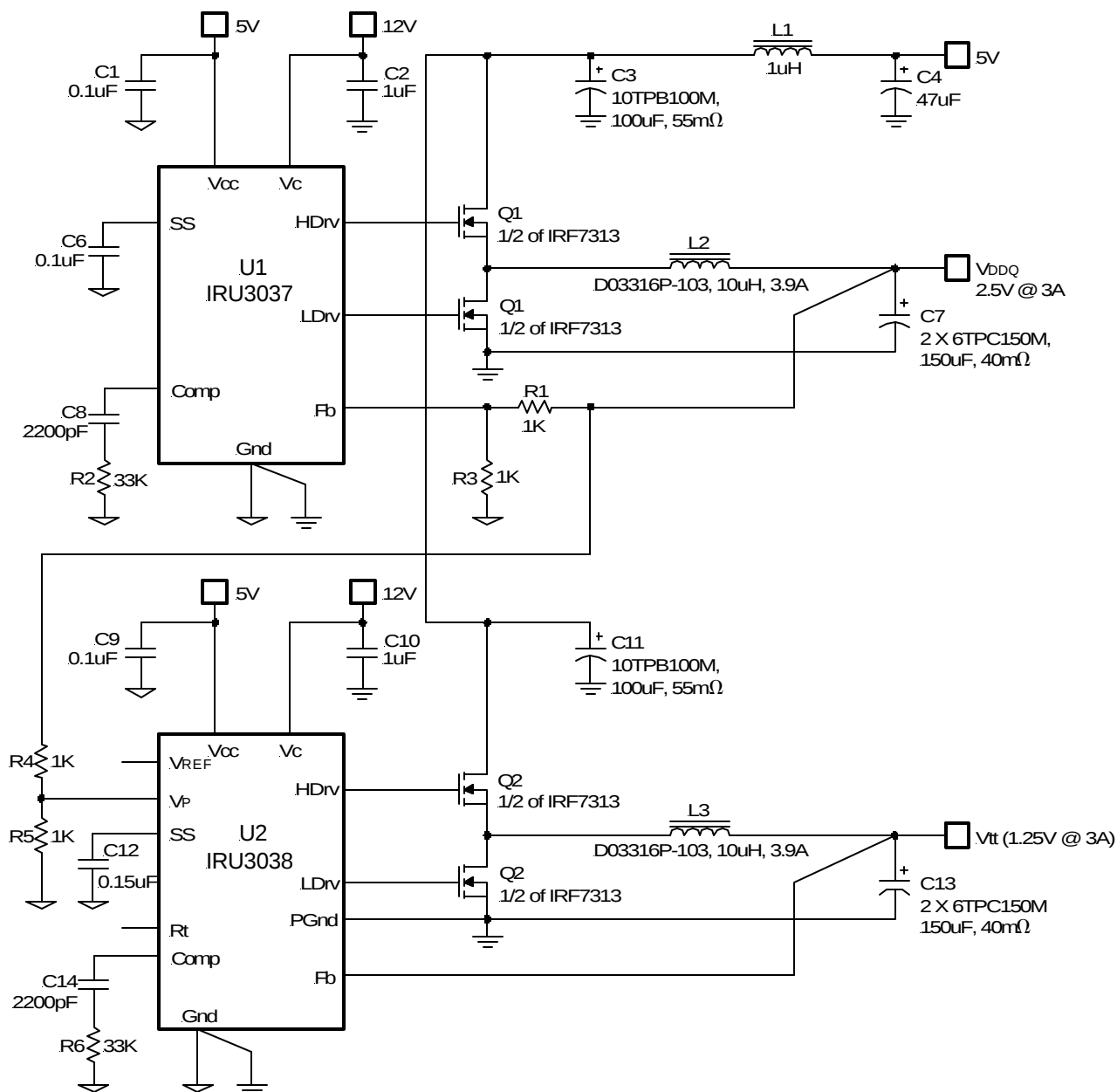
Figure 13 - Typical application of IRU3038 for DDR memory when the termination voltage tracks the core voltage generated by IRU3037 application.
