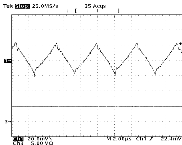
Figure 18 - 3.3V output voltage ripple @ I_{OUT}=5A .
