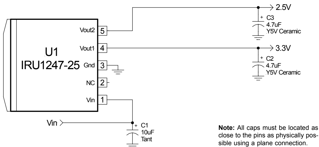
Figure 4 - Typical application of IRU1247-25 in 5-Pin Ultra Thin-Pak and TO-252 (D-Pak) packages.
