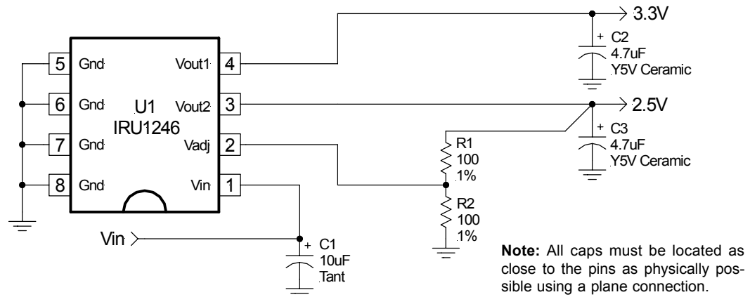
Figure 2 - Typical application of IRU1246 in power 8-Pin SOIC package.
