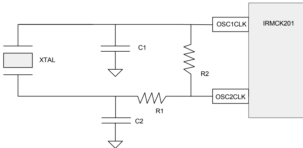
Figure 5. Oscillator Circuit
