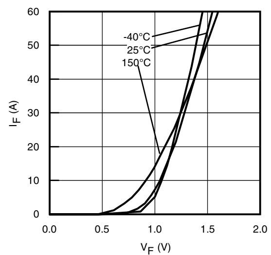
Fig. 8 - Typ. Diode Forward Characteristics tp = 80µs
