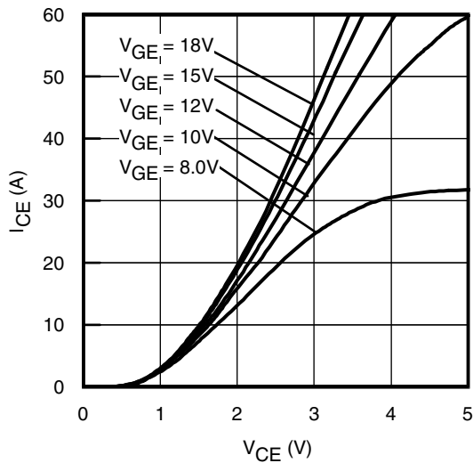
Fig. 7 - Typ. IGBT Output Characteristics T J = 150°C; tp = 80µs
