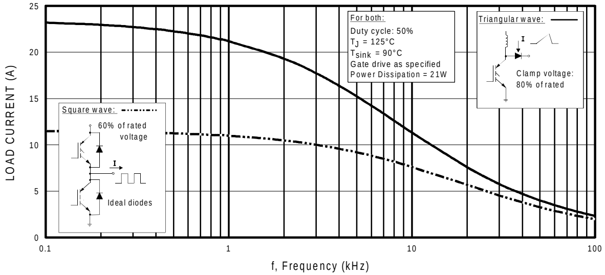
Fig. 1 - Typical Load Current vs. Frequency (For square wave, I = I_{\text{RMS}} of fundamental; for triangular wave, I = I_K )
