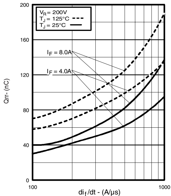
Fig. 21 - Typical Stored Charge vs. di_f/dt
