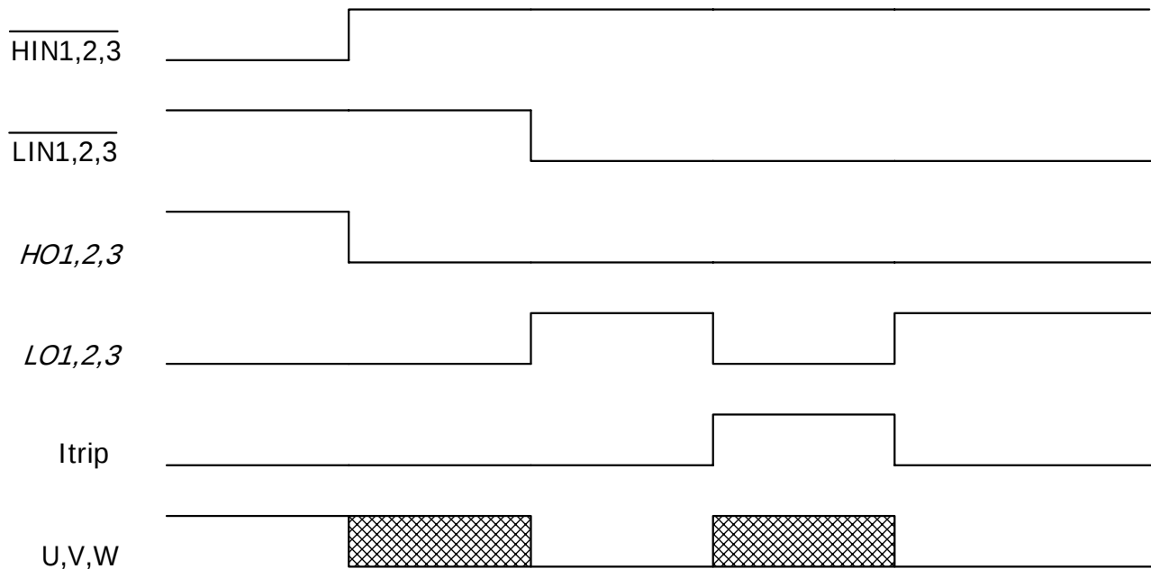
Figure1. Input/Output Timing Diagram
