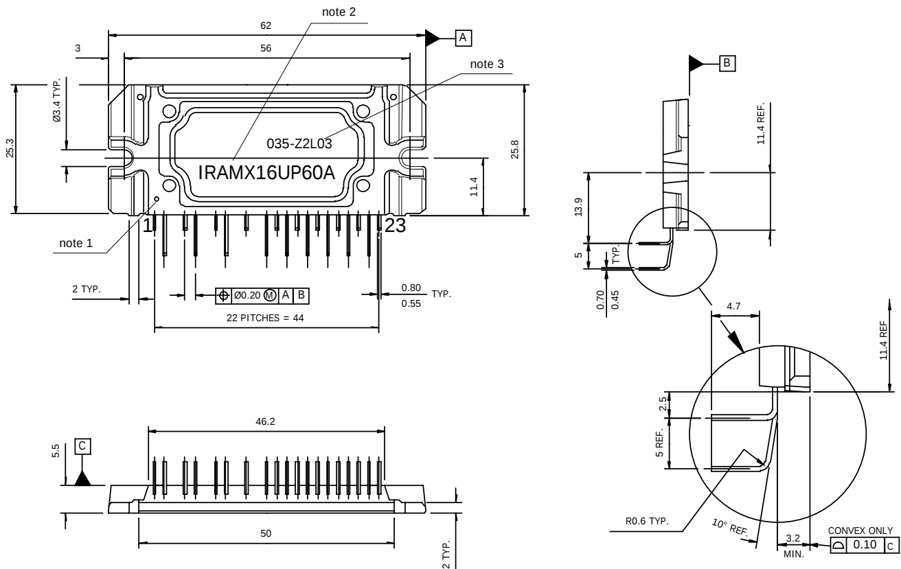
Pin leadforming option -2
