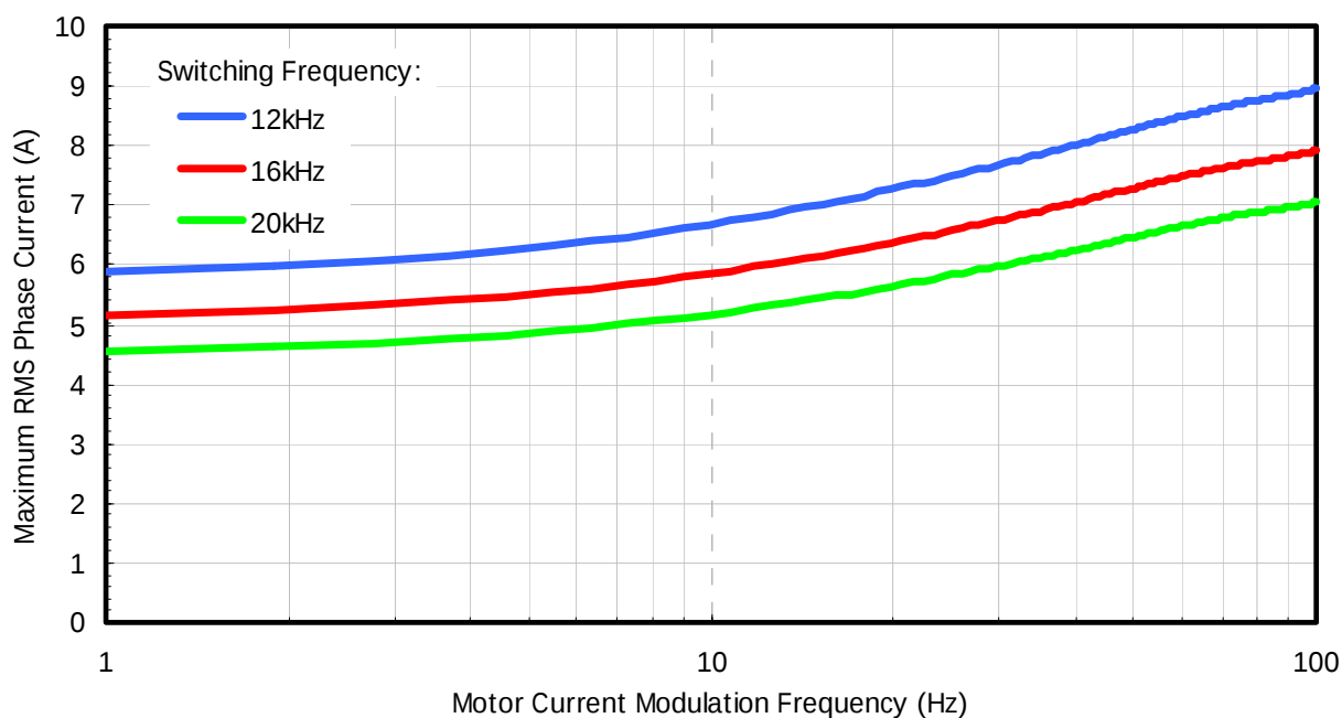
Figure 4. Maximum sinusoidal phase current as function of modulation frequency
