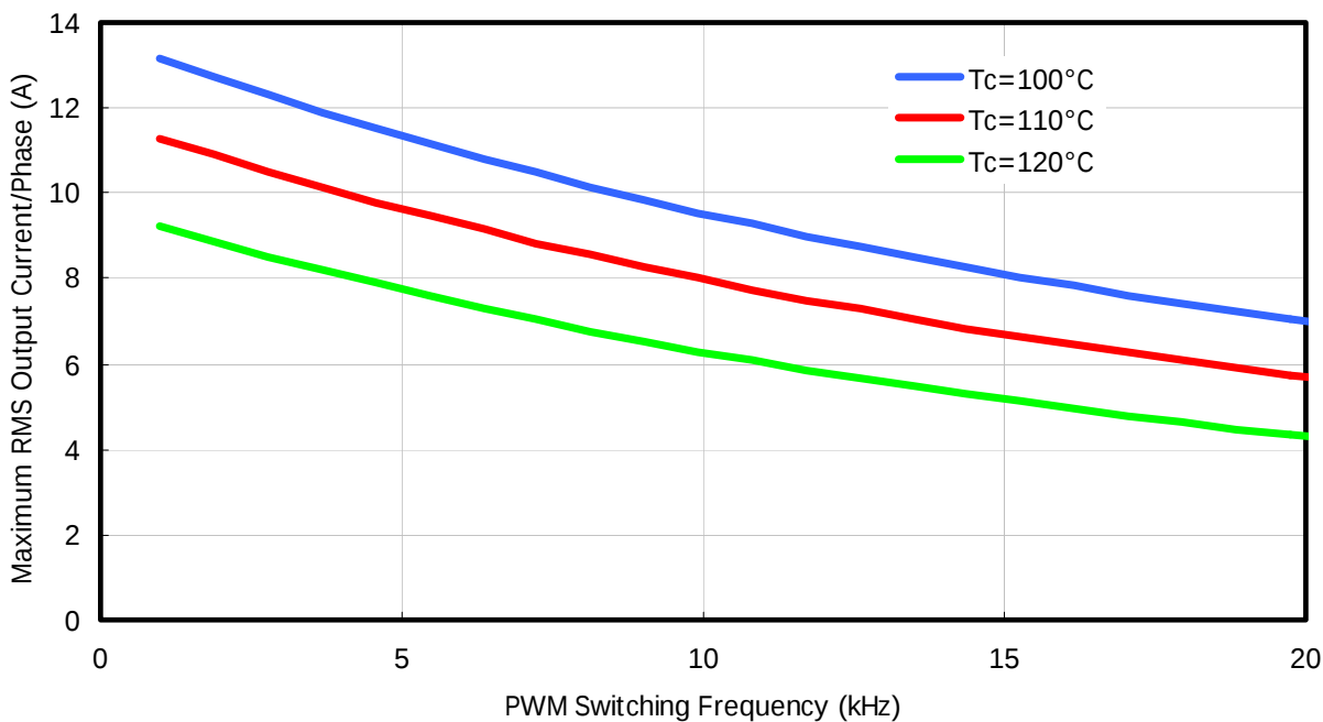
Figure 3. Maximum sinusoidal phase current as function of switching frequency
