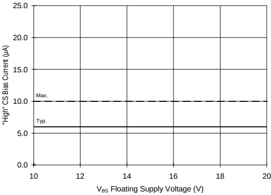
Figure 25B. "High" CS Bias Current vs. Voltage
