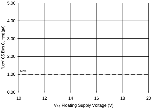
Figure 26B. "Low" CS Bias Current vs. Voltage
