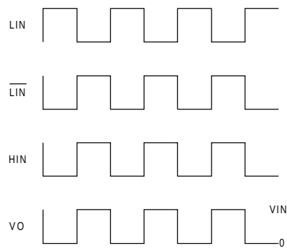
Figure 1. Input/Output Timing Diagram
