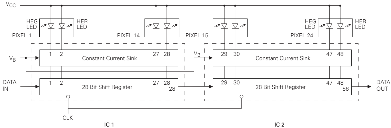
Figure 3. Block Diagram
