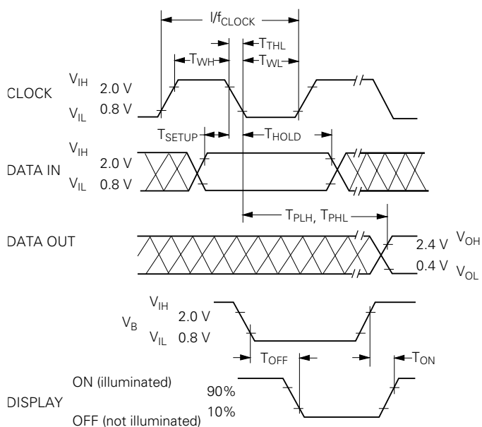
Figure 2. Timing Characteristic
