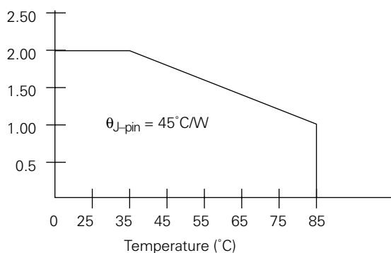
Figure 1. Power Dissipation (Watts)
