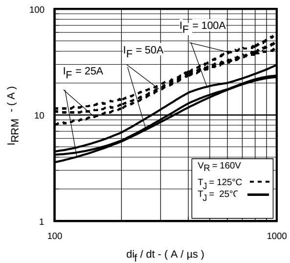
Fig. 6 - Typical Recovery Current Vs. di_f/dt (Per Leg)
