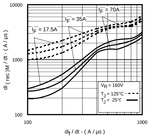
Fig. 8 - Typical di_{(rec)M}/dt Vs. di_f/dt (Per Leg)
