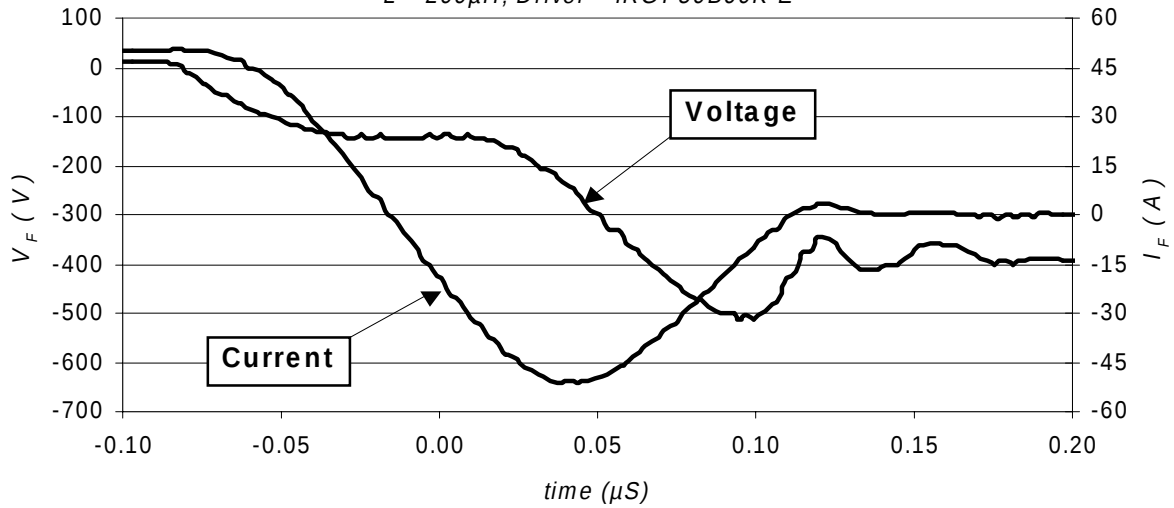
Fig. 1 - Typical Diode Recovery Waveform
