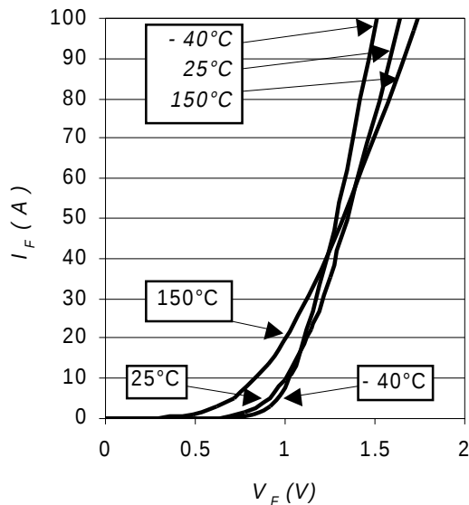
Fig. 2 - Typical Diode Forward Characteristics
