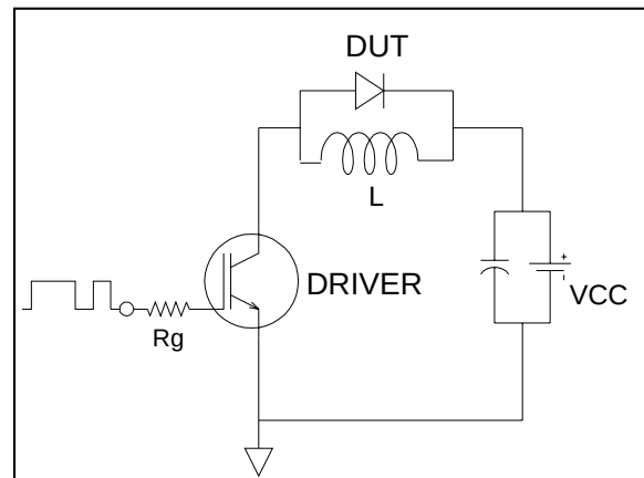
Fig. 3 - Diode Recovery Circuit
