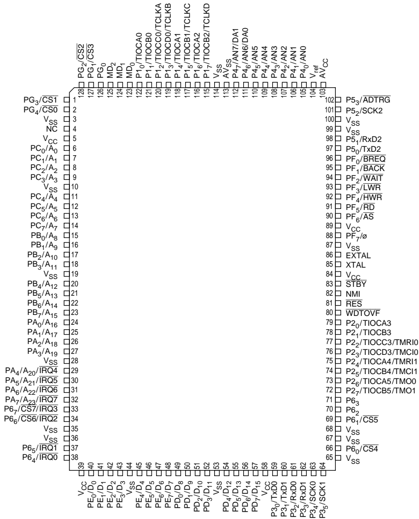
128-Pin Plastic QFP (FP-128: Top View)
