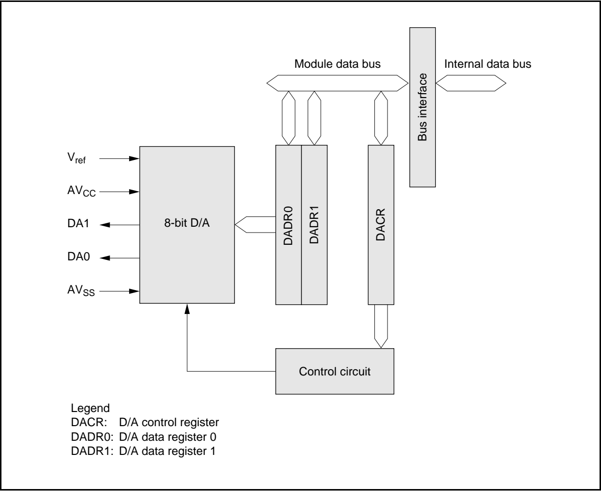
Block Diagram of D/A Converter
