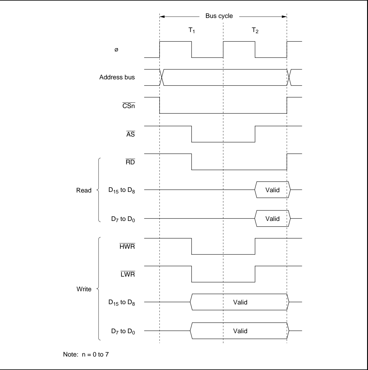
Basic Bus Timing (Word Access to 16-Bit 2-State Access Space)
