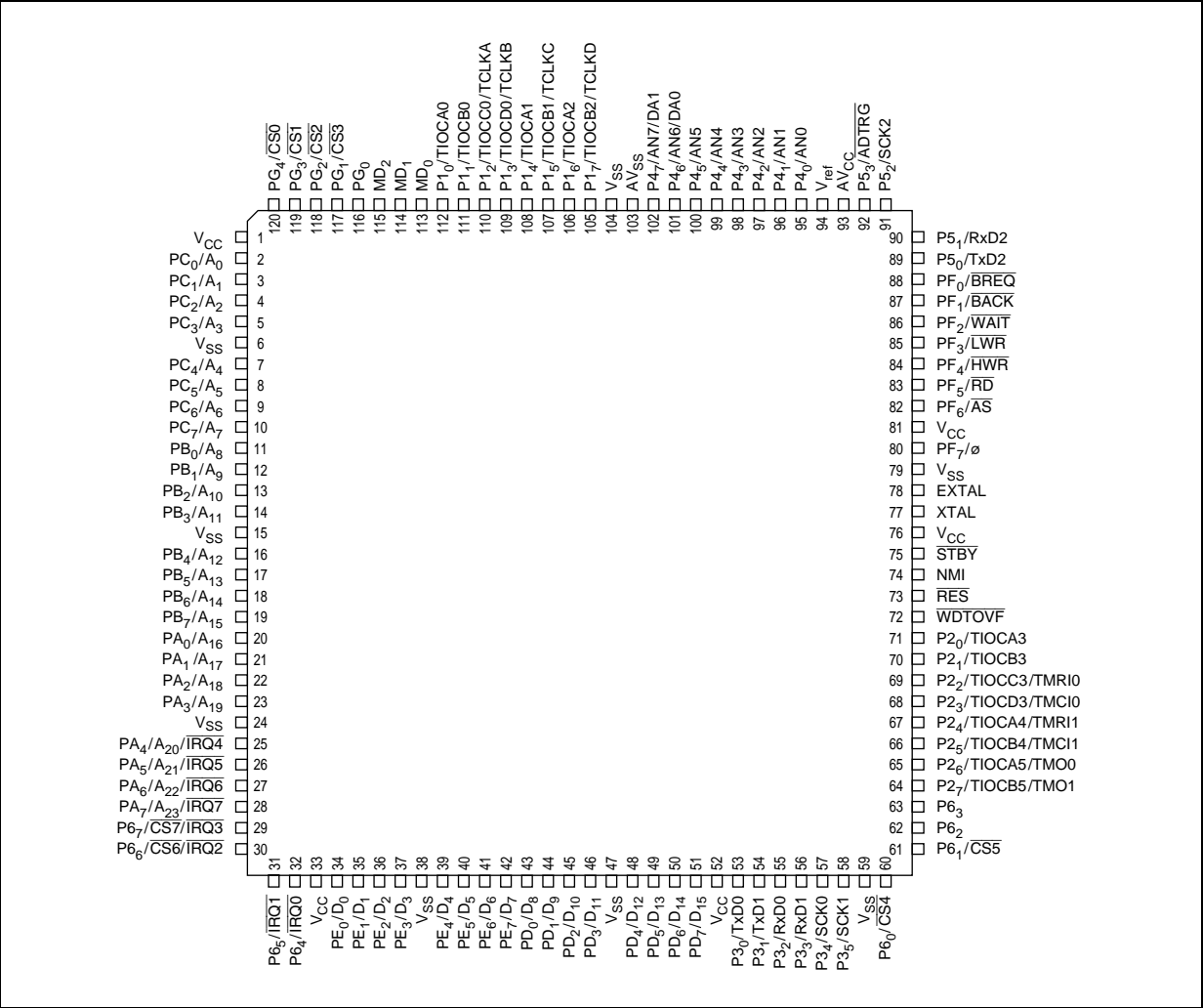
120-Pin Plastic TQFP (TFP-120: Top View)
