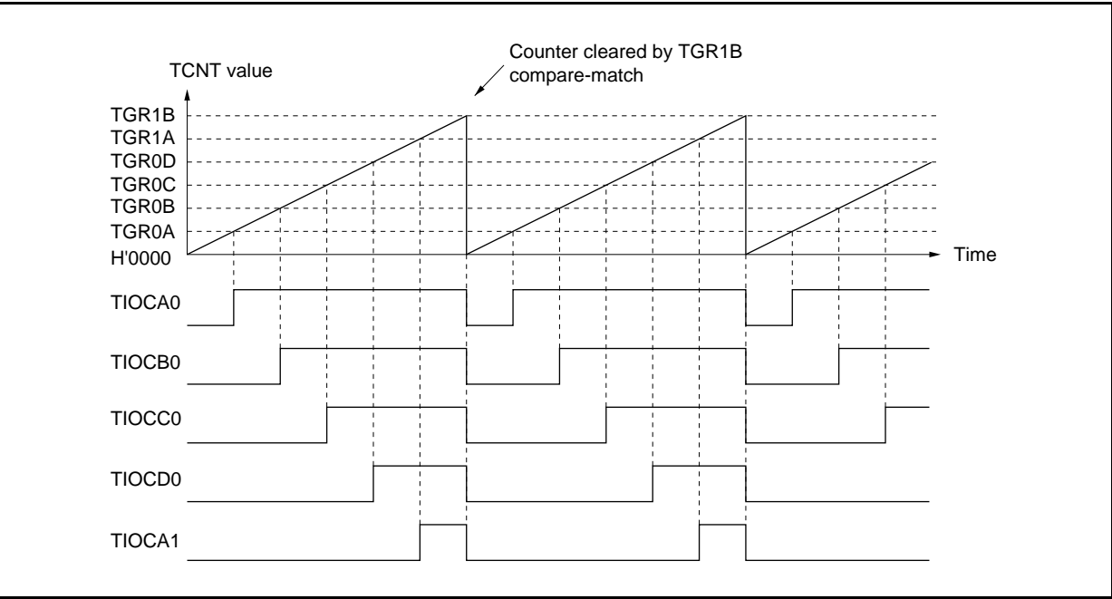
Operation in PWM Mode 2
