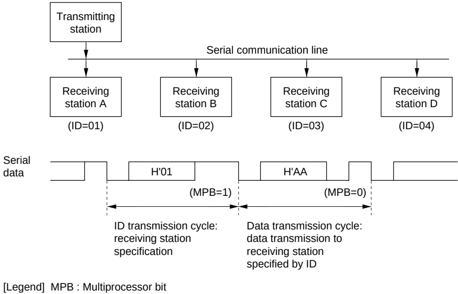
Figure 22.10 Example of Inter-Processor Communication Using Multiprocessor Format (Transmission of Data H'AA to Receiving Station A)
