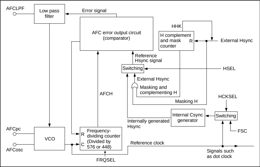
Figure 27.20 AFC Configuration
