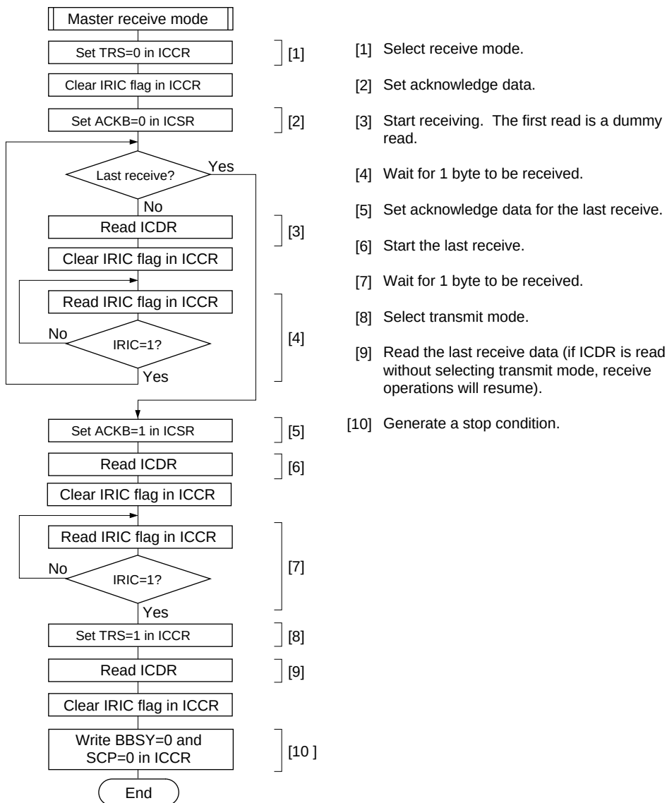
Figure 23.15 Flowchart for Master Receive Mode (Example)
