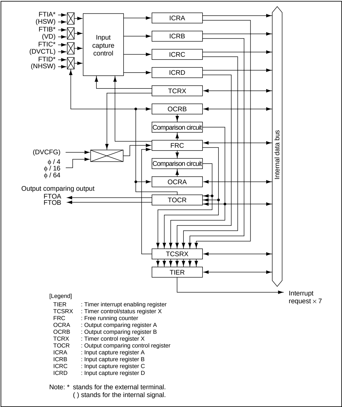
Figure 16.1 Block Diagram of Timer X1
