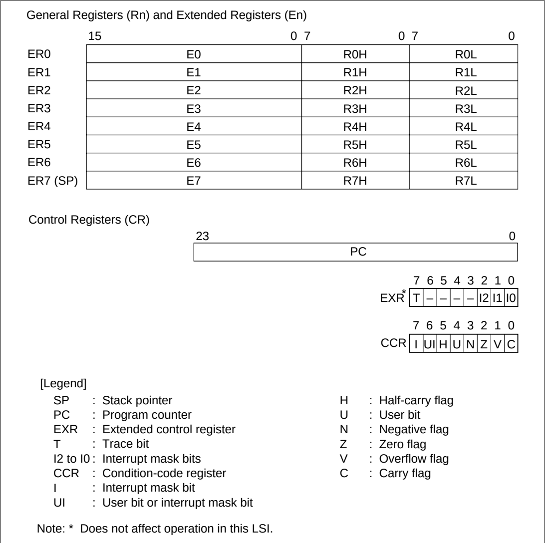
Figure 2.7 CPU Registers
