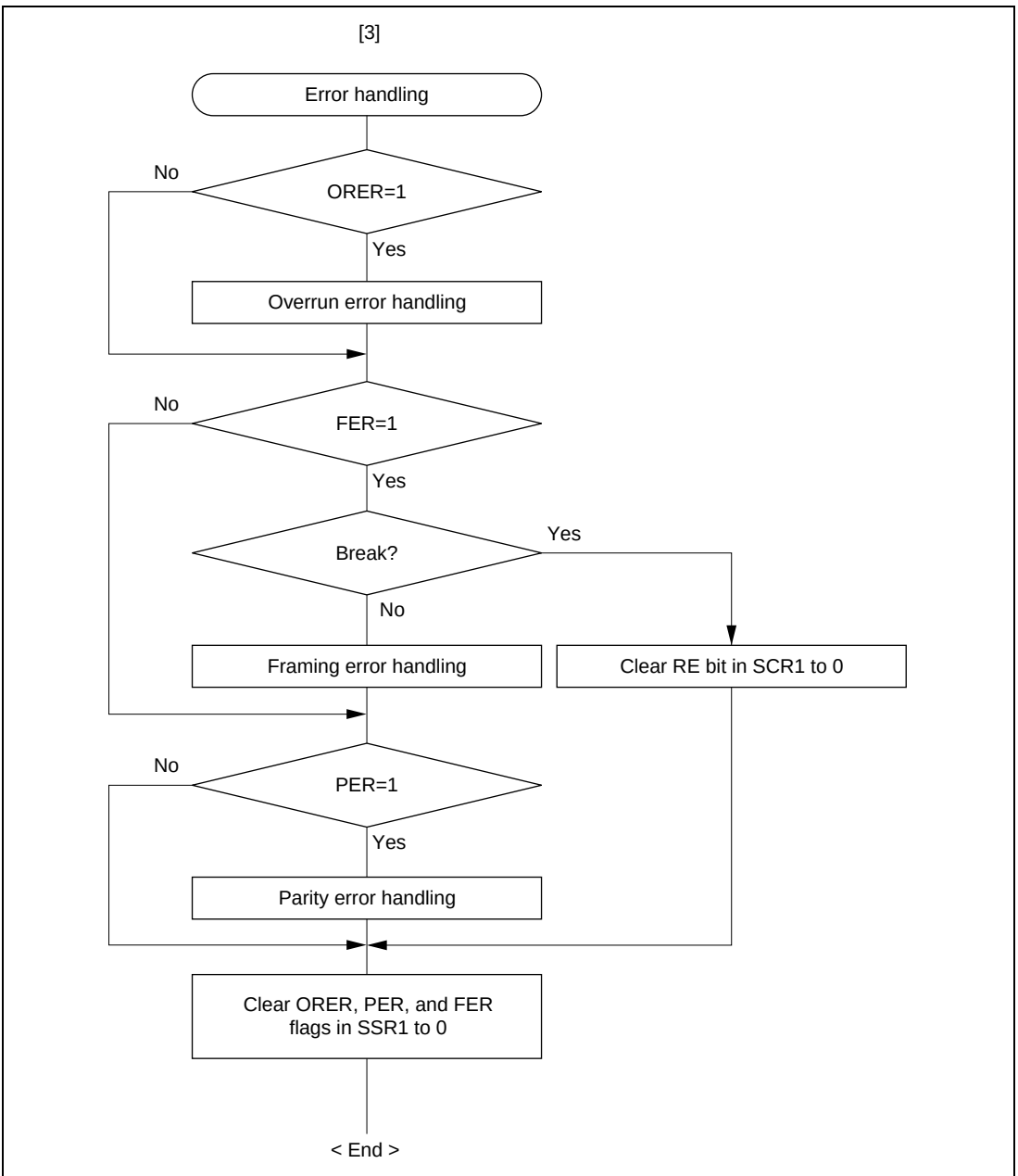
Figure 22.8 Sample Serial Reception Data Flowchart (2)
