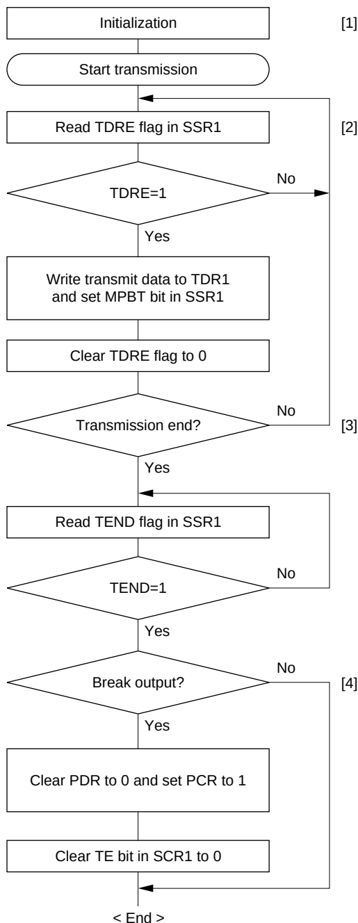
Figure 22.11 Sample Multiprocessor Serial Transmission Flowchart
