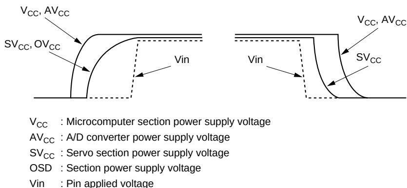
Figure E.1 Power Supply Rise and Fall Order
