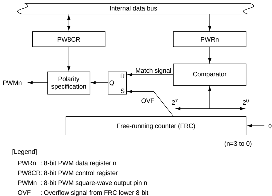
Figure 18.1 Block Diagram of 8-Bit PWM (1 channel)
