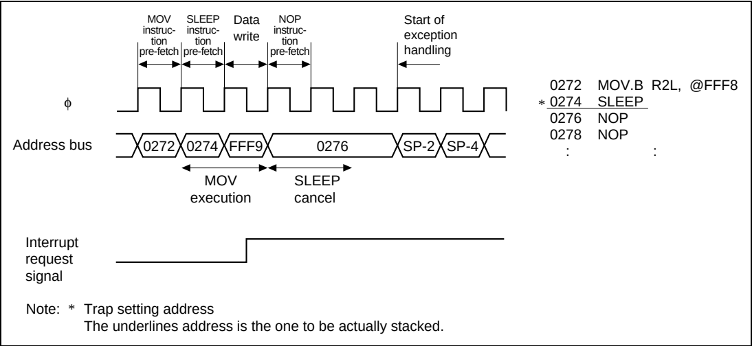
Figure 25.16 SLEEP Instruction (1)
