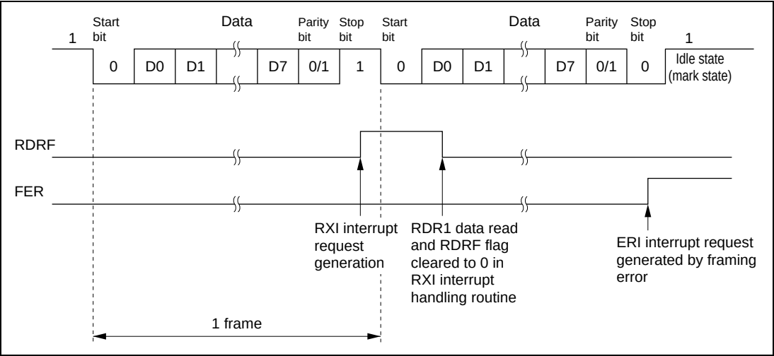
Figure 22.9 Example of SCI Operation in Reception (Example with 8-Bit Data, Parity, One Stop Bit)
