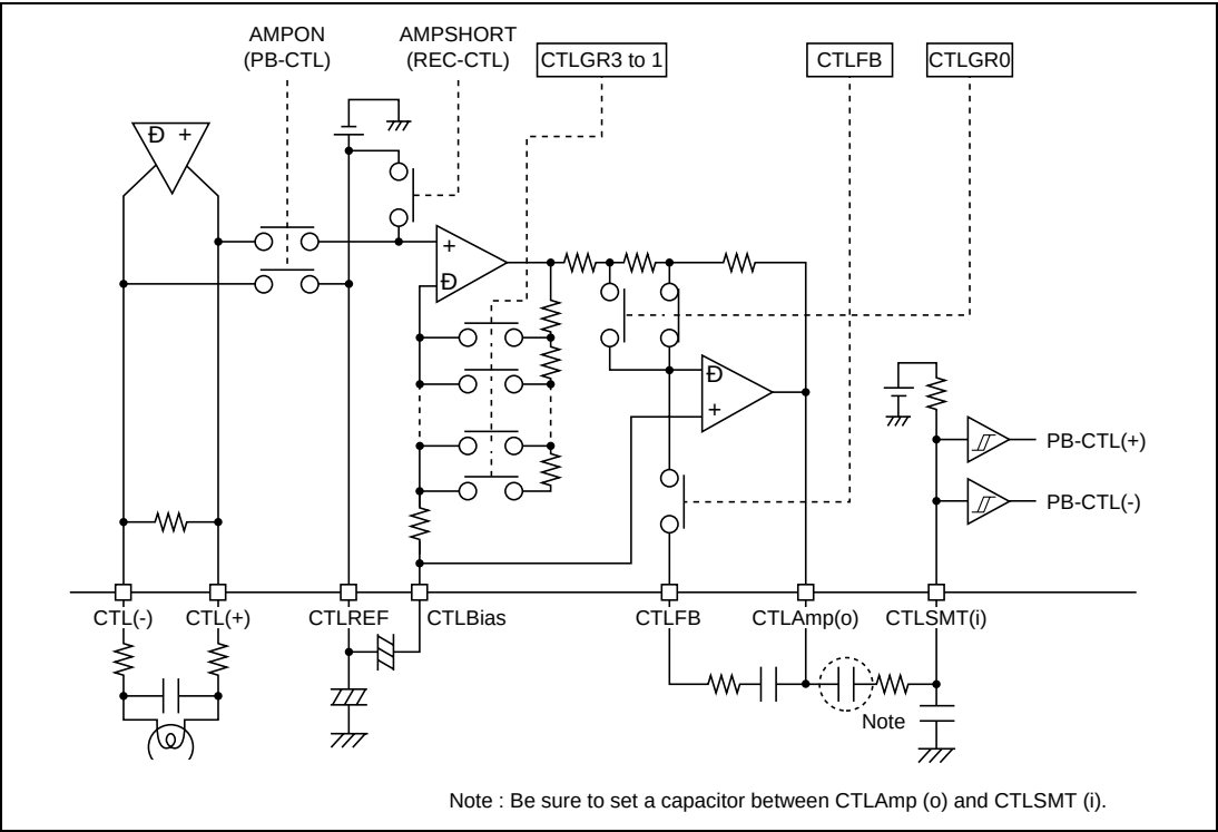
Figure 26.52 Block Diagram of CTL Input Amplifier
