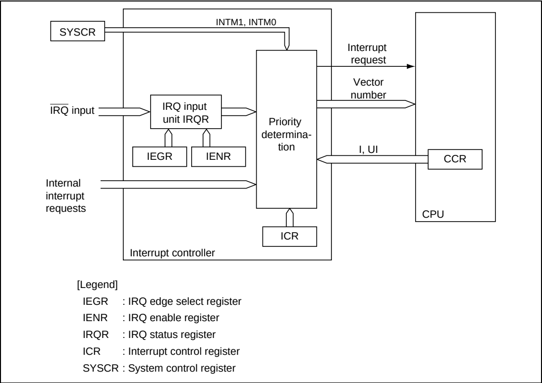
Figure 6.1 Block Diagram of Interrupt Controller
