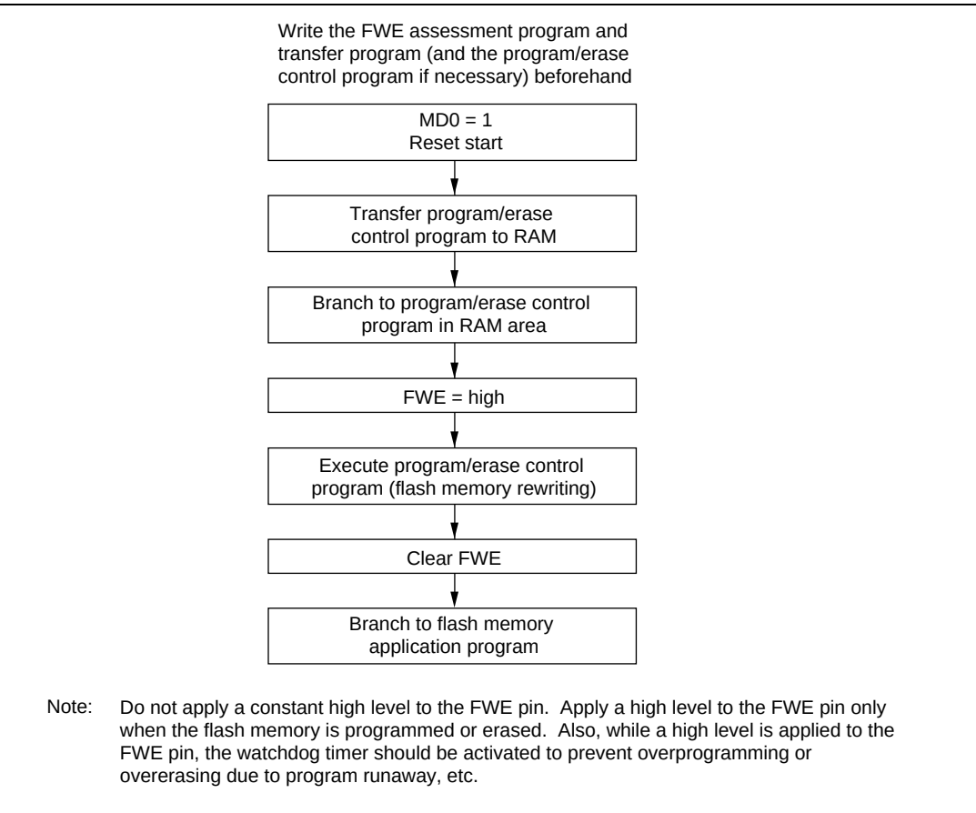
Figure 7.11 User Program Mode Execution Procedure (Preliminary)
