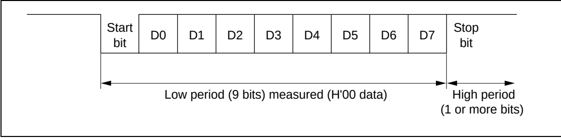
Figure 7.9 Automatic SCI Bit Rate Adjustment
