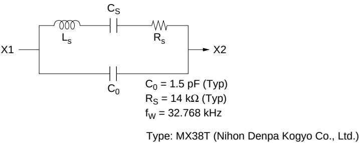
Figure 9.9 32.768 kHz Crystal Resonator Equivalent Circuit
