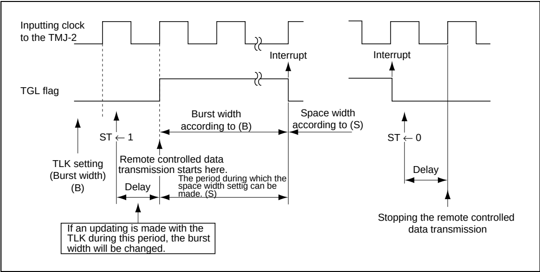
Figure 13.4 Controls of the Remote Controlled Data Transmission
