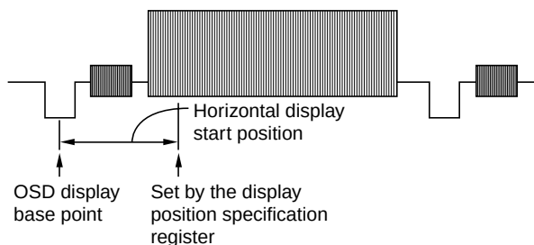
Figure 29.11 Base Point for Horizontal Display Start Position
