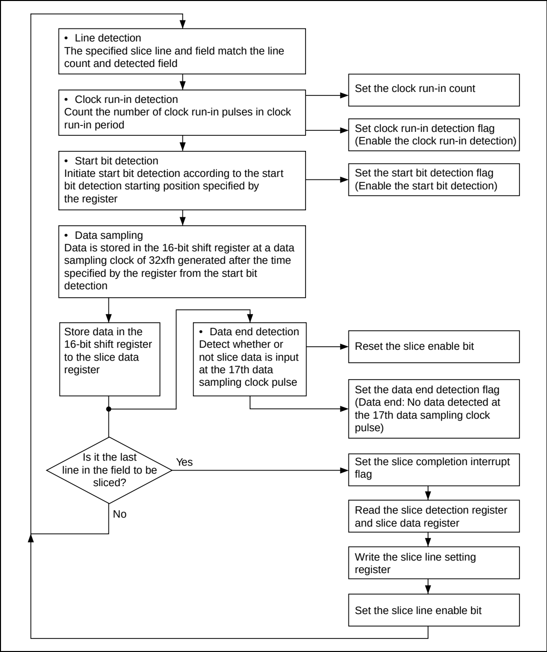
Figure 28.11 Slice Sequence
