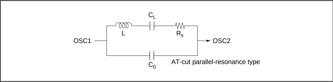
Figure 9.3 Crystal Resonator Equivalent Circuit
