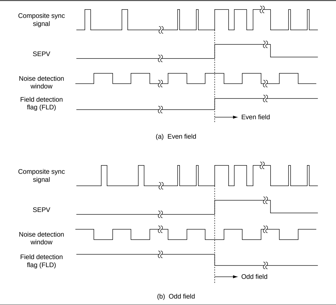
Figure 26.74 Field Detection
