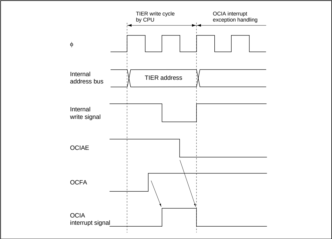
Figure 6.9 Contention between Interrupt Generation and Disabling
