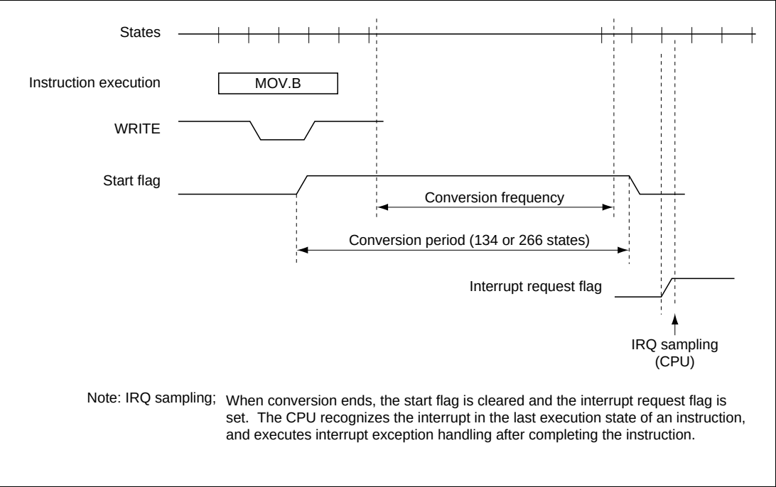
Figure 24.2 Internal Operation of A/D Converter
