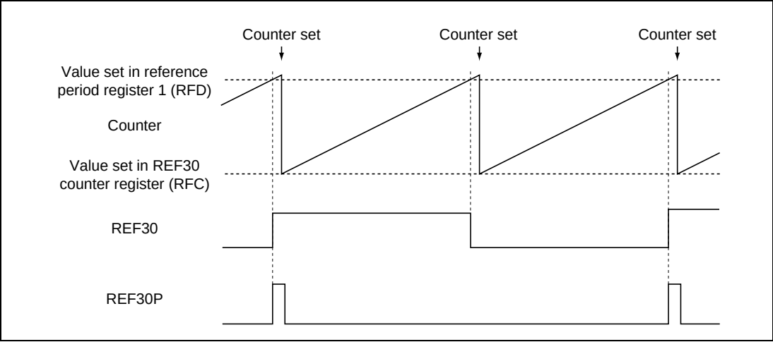
Figure 26.8 REF30 Signals in Playback Mode
