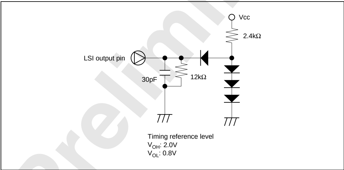
Figure 30.17 Output Load Conditions
