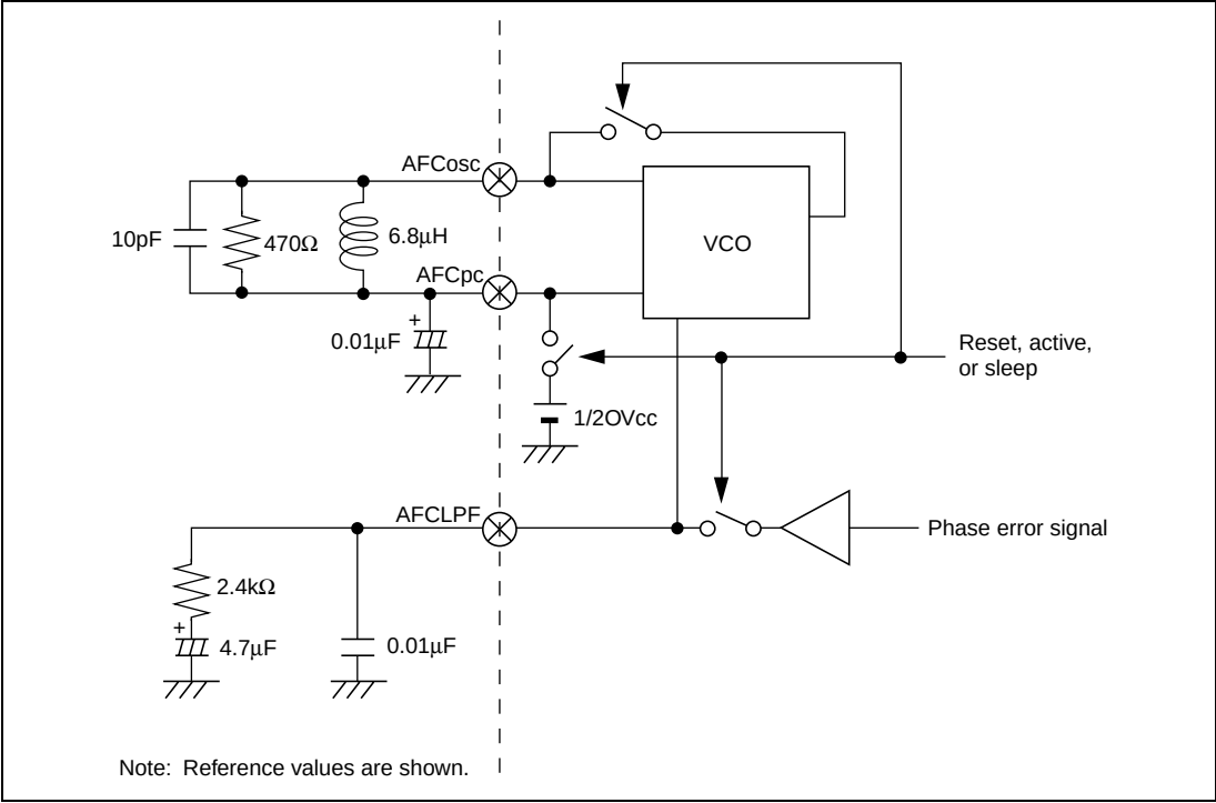
Figure 27.21 Circuit Example for a 576 × fh Reference Clock
