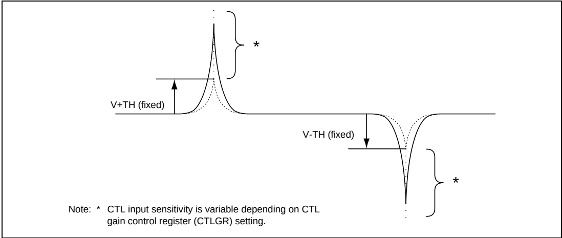
Figure 26.53 CTL Input Pulse Gain Control
