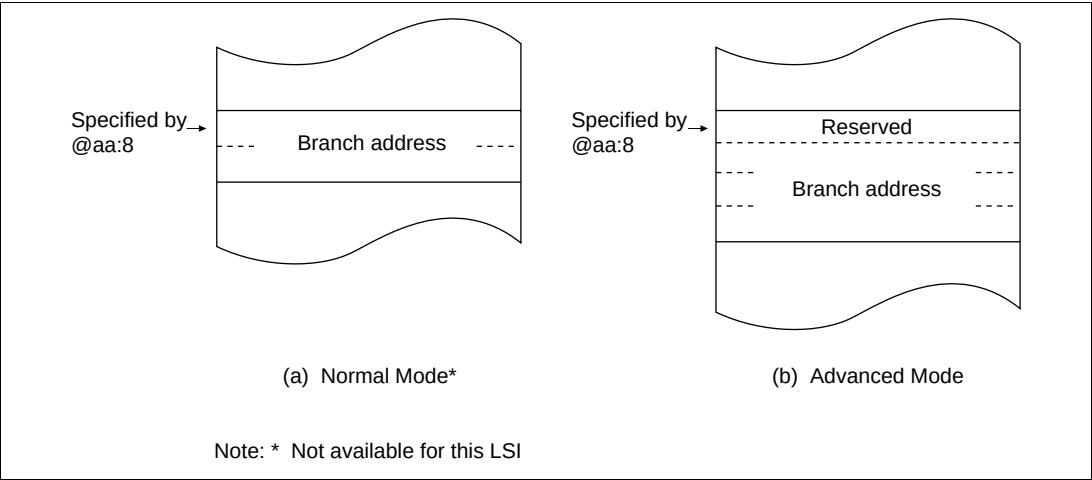
Figure 2.14 Branch Address Specification in Memory Indirect Mode
