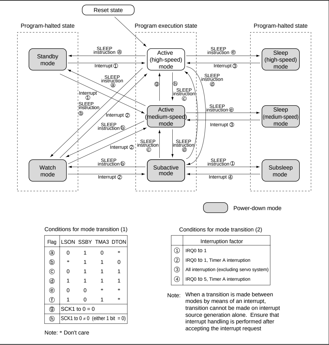
Figure 4.1 Mode Transitions
