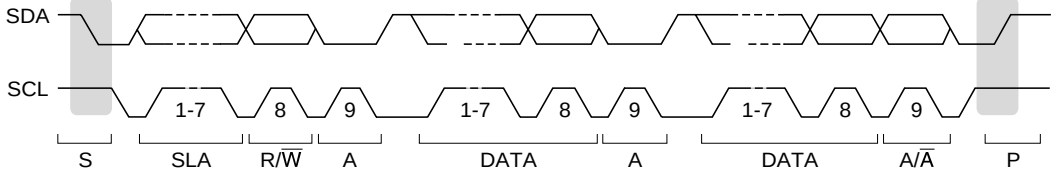
Figure 23.5 I²C Bus Timing
