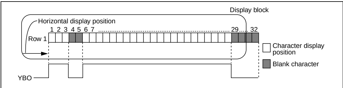
Figure 29.15 YBO Output Example
