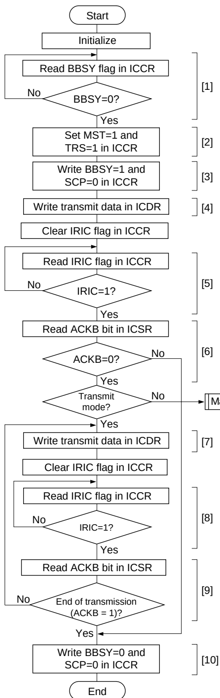
Figure 23.14 Flowchart for Master Transmit Mode (Example)
