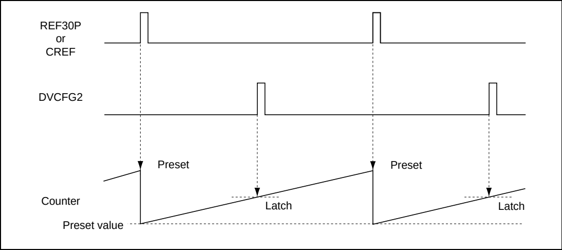
Figure 26.36 Capstan Phase Control in Record Mode
