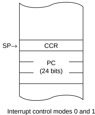
Figure 5.5 Stack Status after Exception Handling (Advanced Mode)
