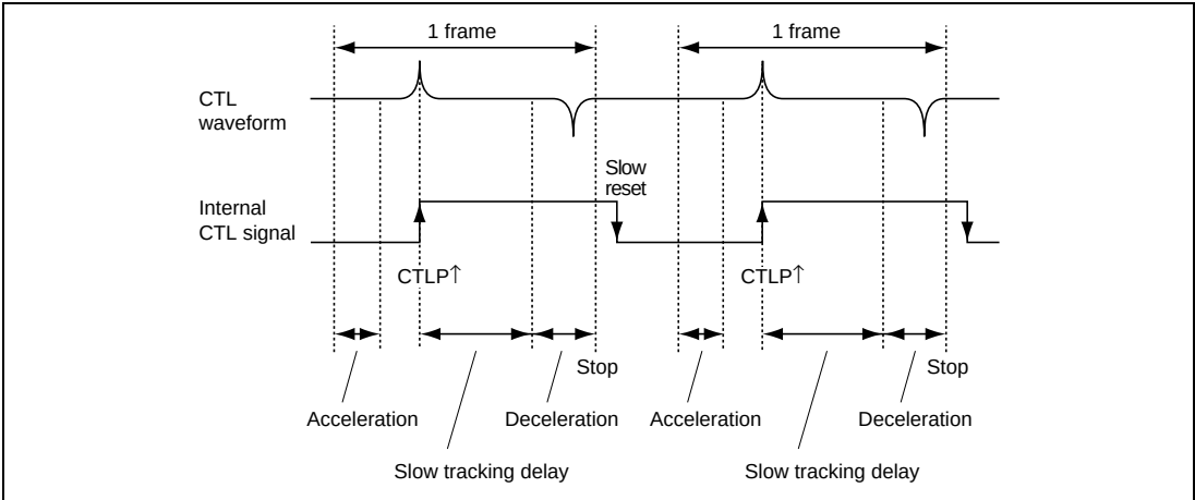
Figure 26.54 PB-CTL Waveform in Slow Mode Operation
