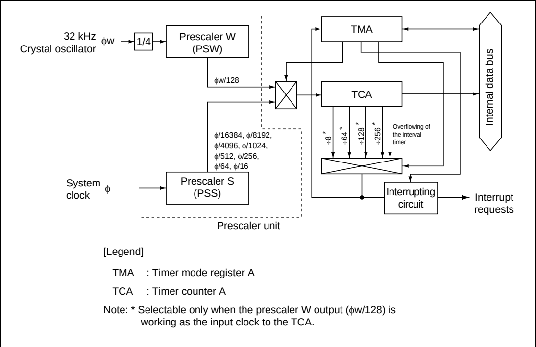
Figure 11.1 Block Diagram of Timer A
