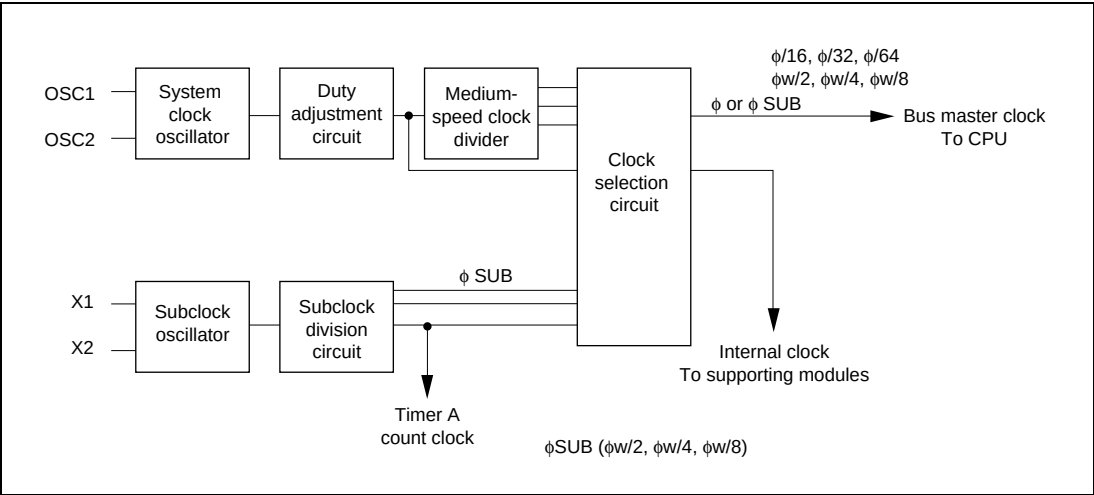
Figure 9.1 Block Diagram of Clock Pulse Generator
