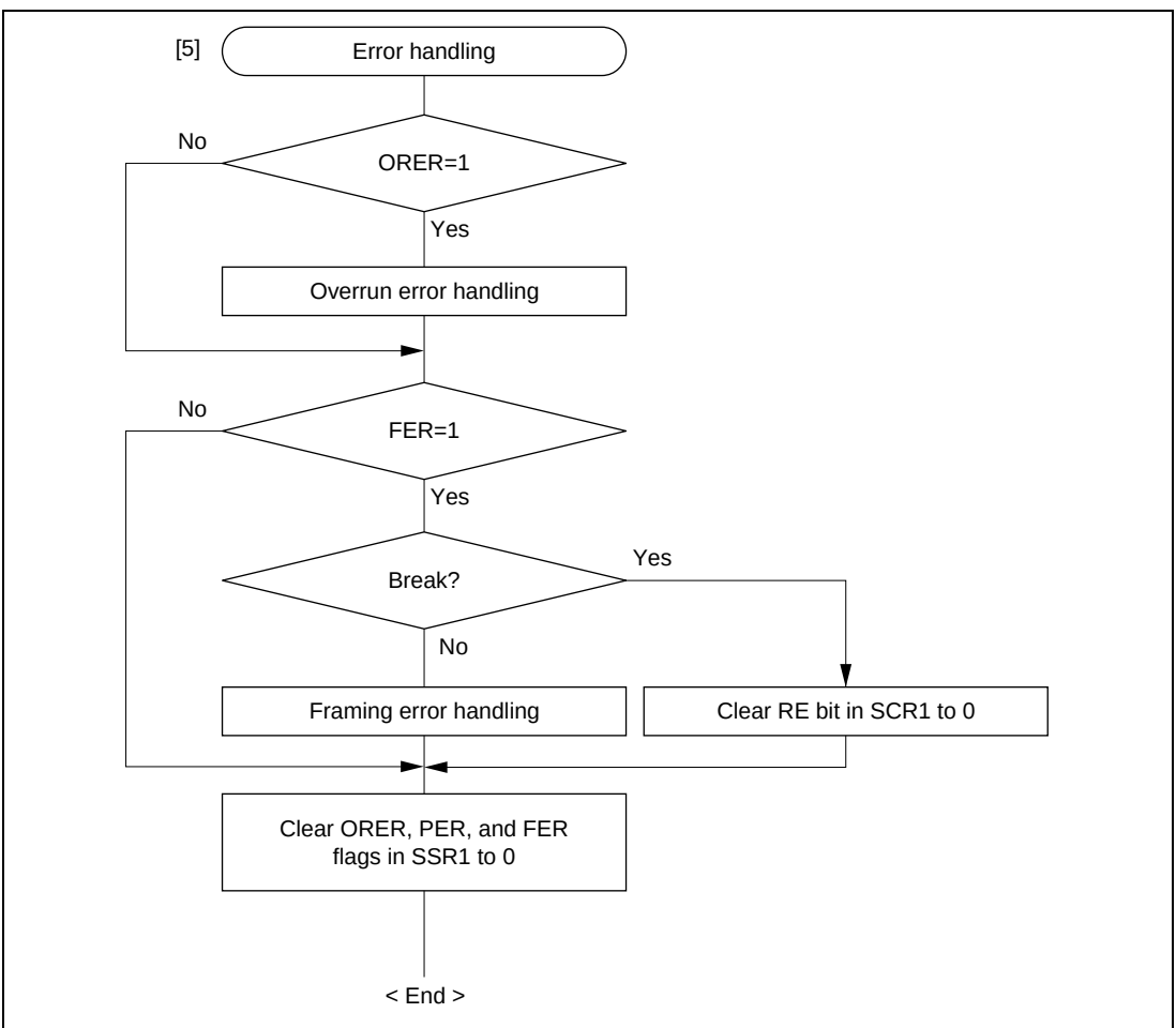
Figure 22.14 Sample Multiprocessor Serial Reception Flowchart (2)
