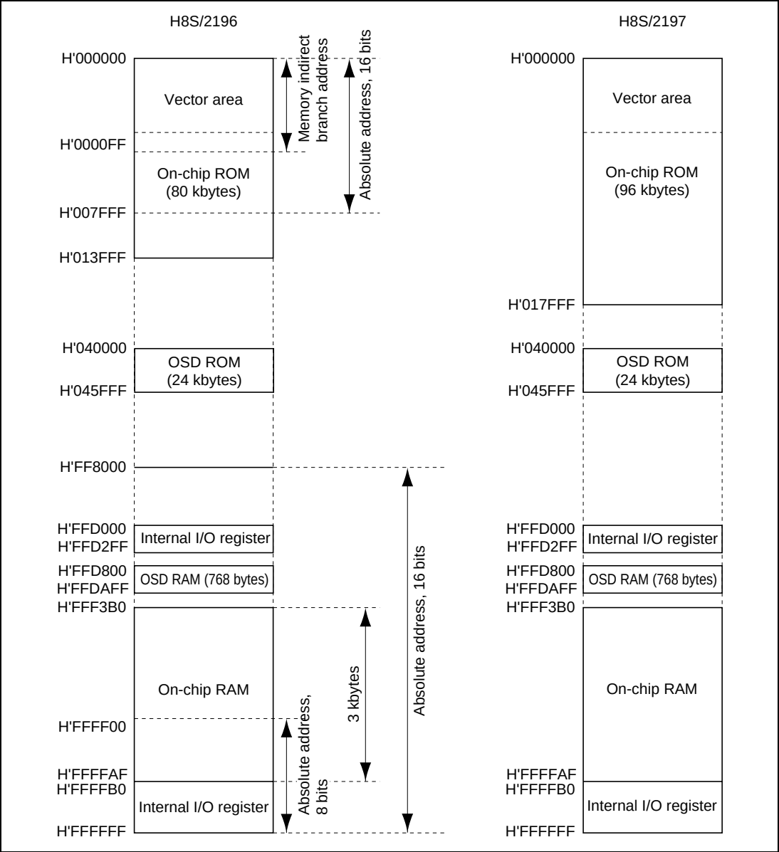
Figure 3.1 Address Map (1)
