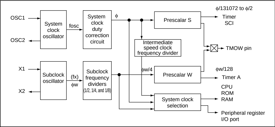
Figure 21.2 Clock Supply
