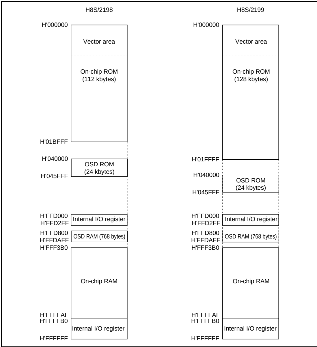
Figure 3.2 Address Map (2)
