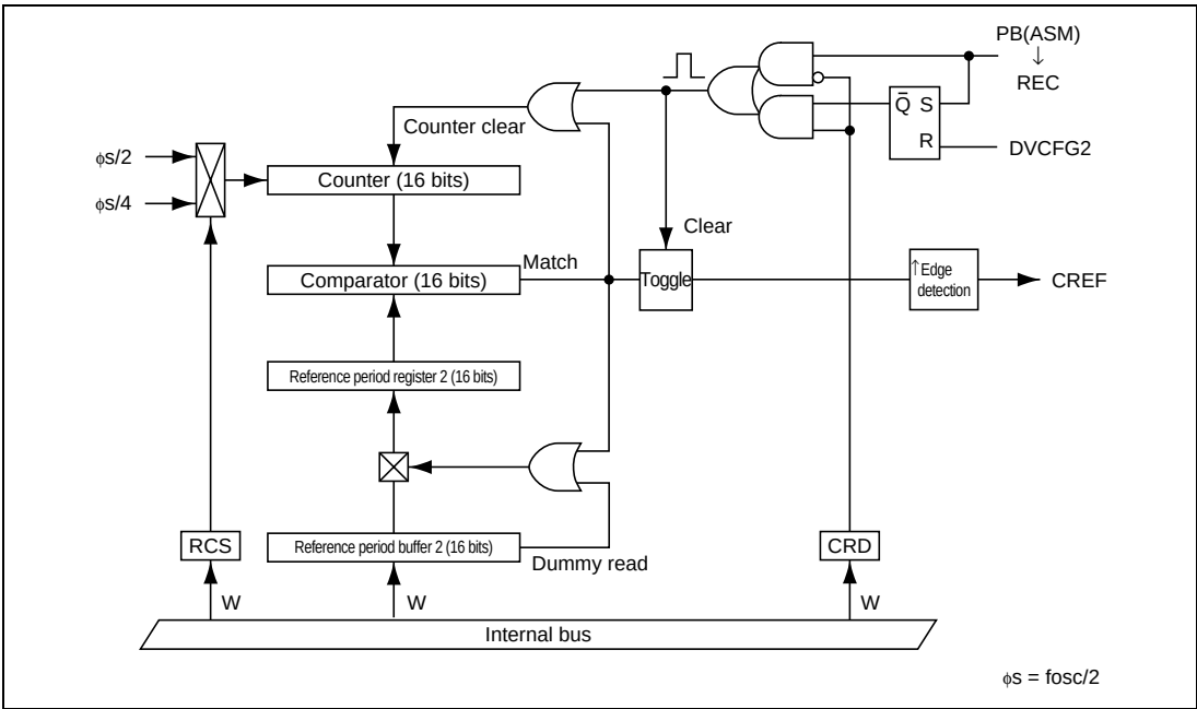
Figure 26.7 Block Diagram of CREF Signal Generator
