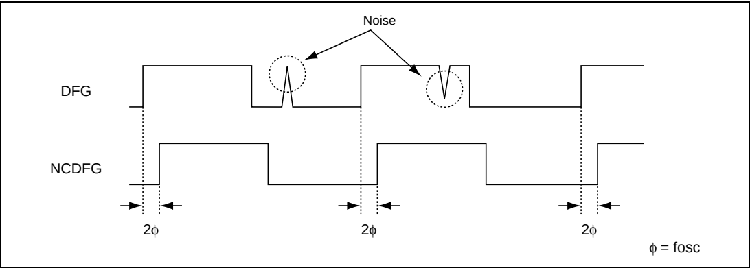
Figure 26.71 NCDFG Signal
