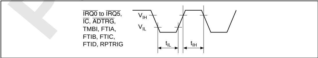
Figure 30.14 Input Timing
