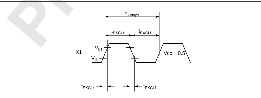
Figure 30.11 Subclock Input Timing
