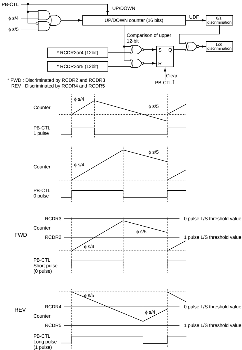
Figure 26.56 Duty Discriminator
