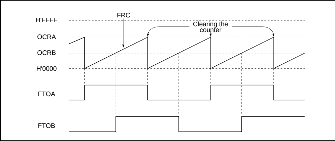
Figure 16.12 Pulse Outputting Example
