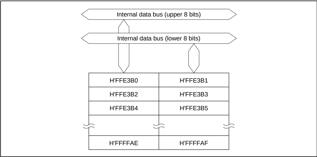
Figure 8.1 Block Diagram of RAM (H8S/2199)
