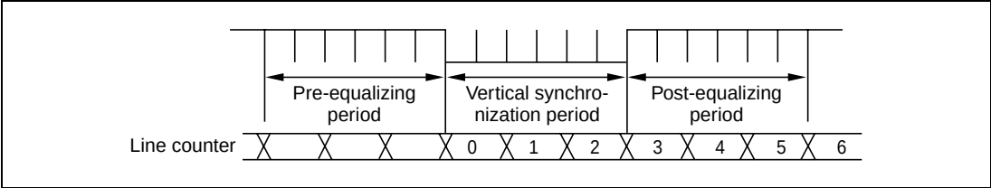
Figure 29.10 Base Point for Vertical Display Start Positions
