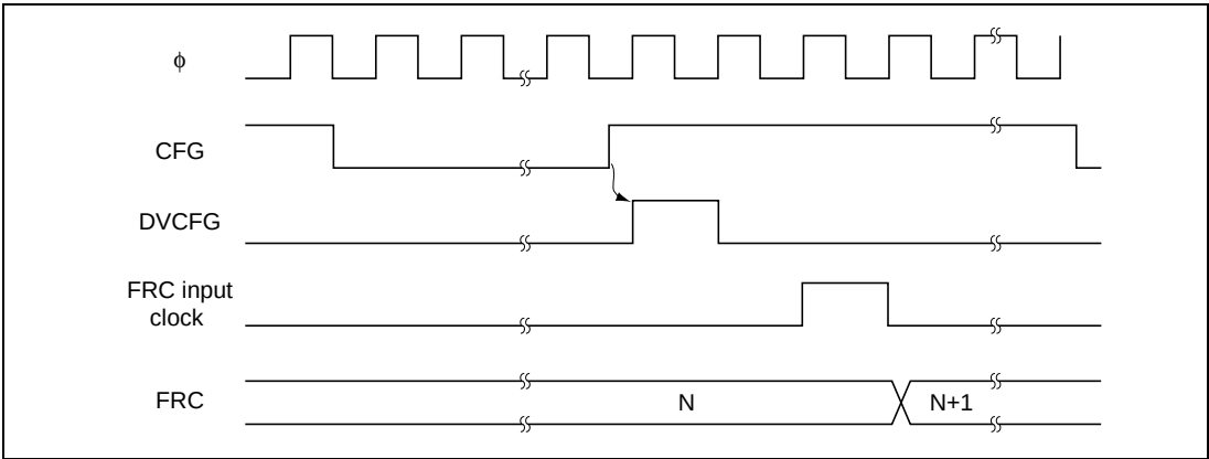
Figure 16.4 Count Timing for CFG Clock Operation
