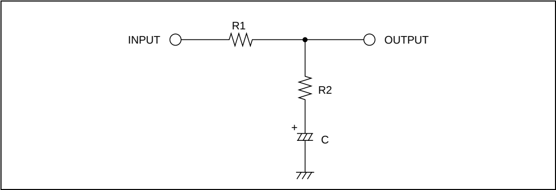
Figure 26.40 Lag-Lead Filter
