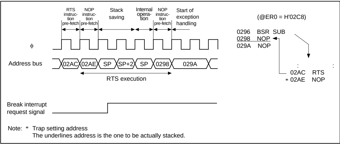
Figure 25.15 RTS Instruction
