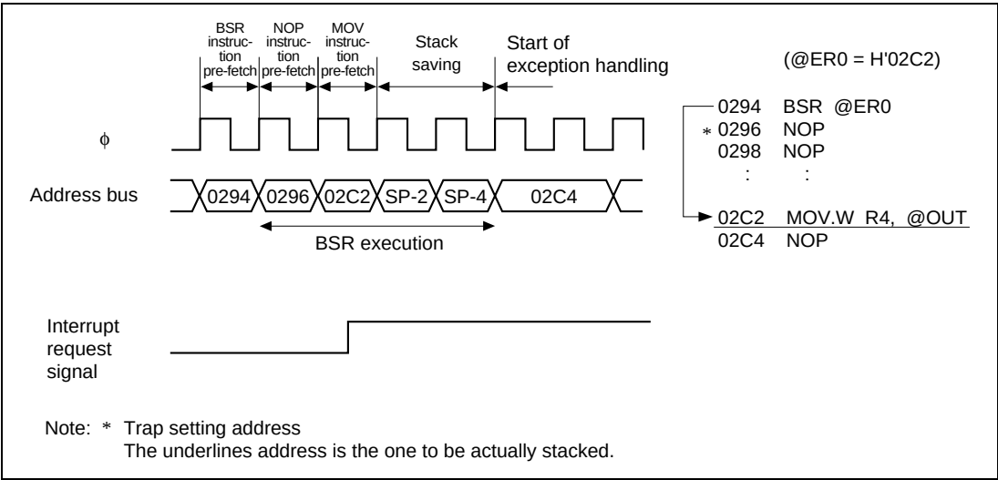
Figure 25.10 BSR Instruction (8-bit Displacement)
