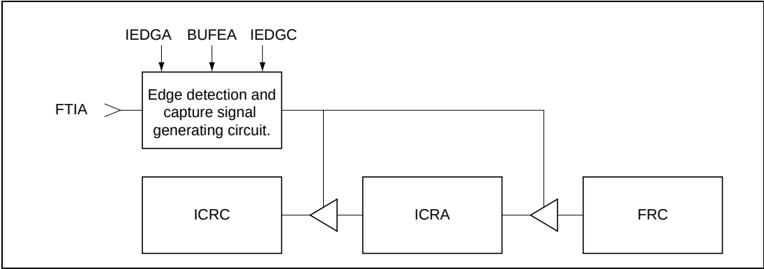
Figure 16.2 Buffer Operation (Example)
