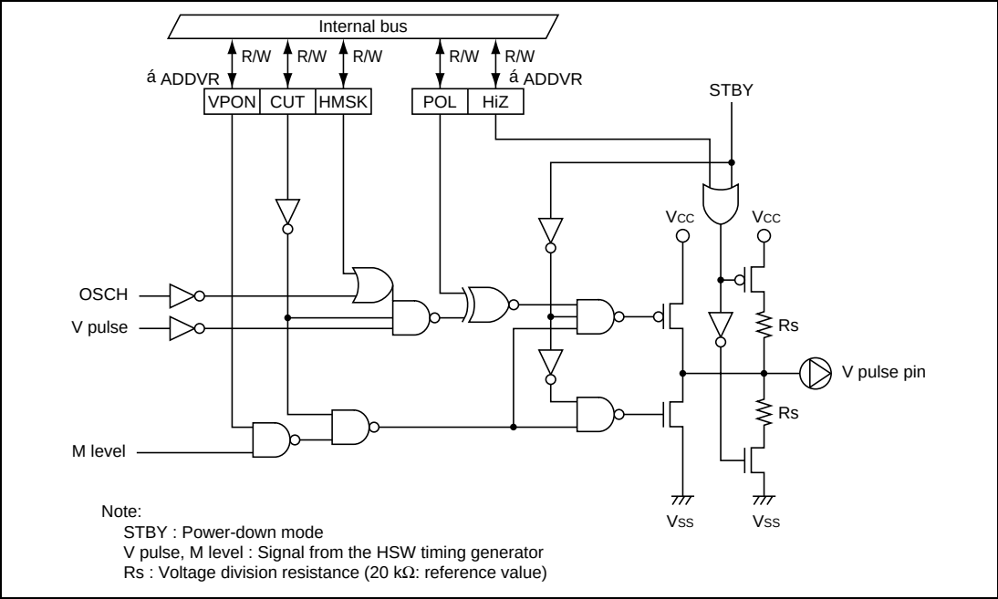
Figure 26.44 Additional V Pulse Pin
