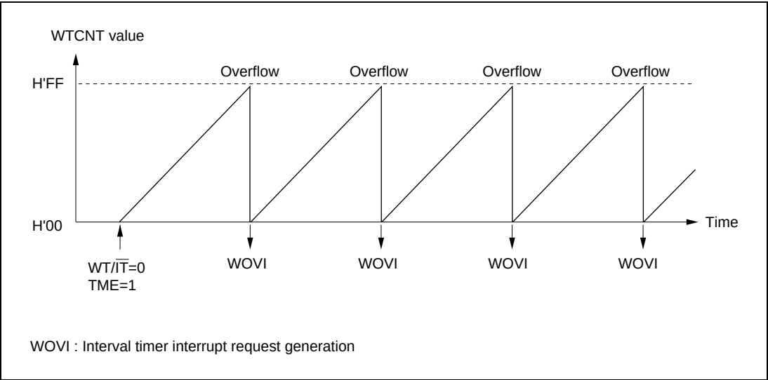
Figure 17.4 Operation in Interval Timer Mode
