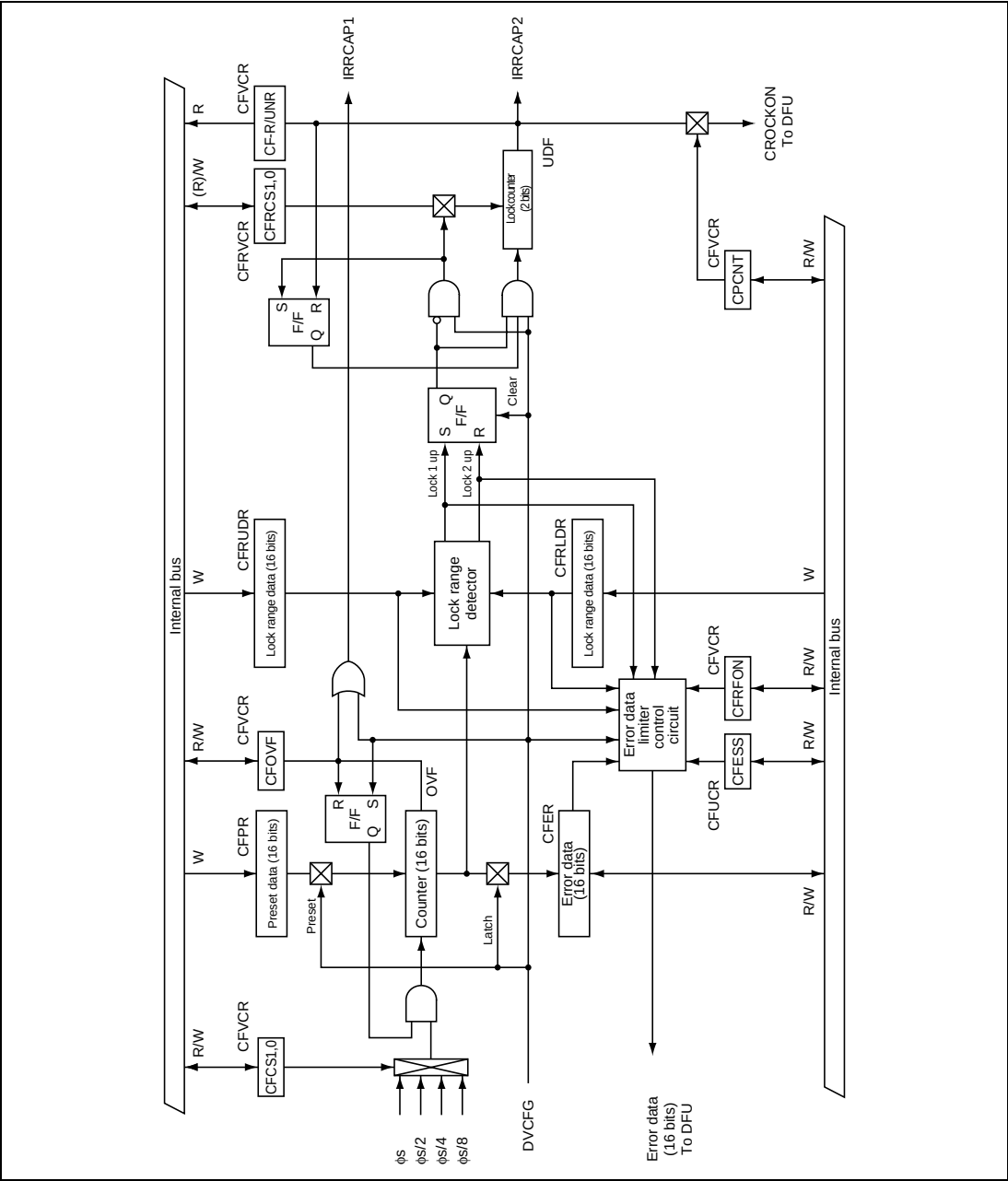
Figure 26.32 Block Diagram of Capstan Speed Error Detector
