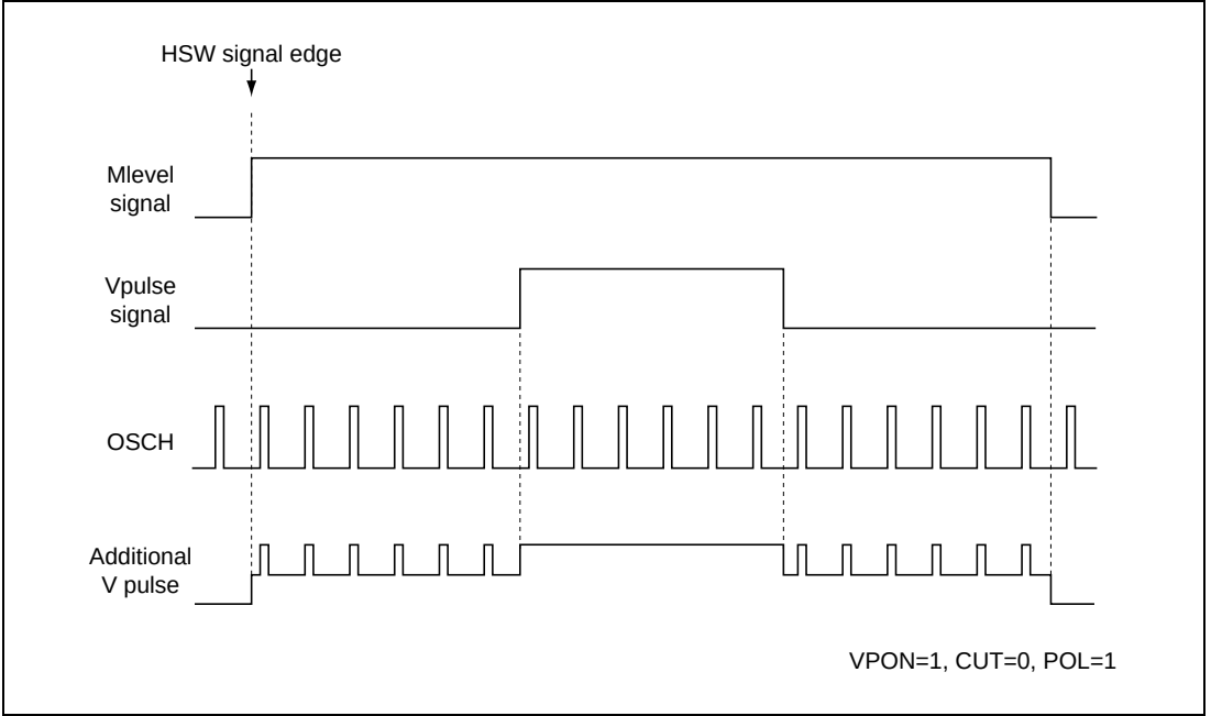
Figure 26.45 Additional V Pulse when Positive Polarity Is Specified
