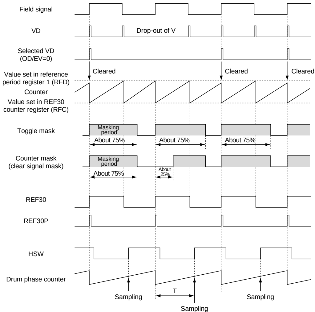
Figure 26.10 Generation of the Reference Signal when in REC (V Dropped Out)
