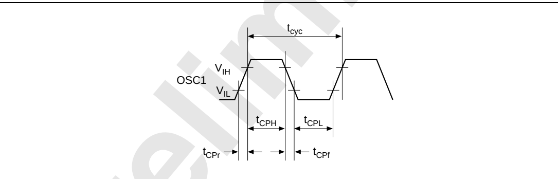
Figure 30.10 System Clock Timing
