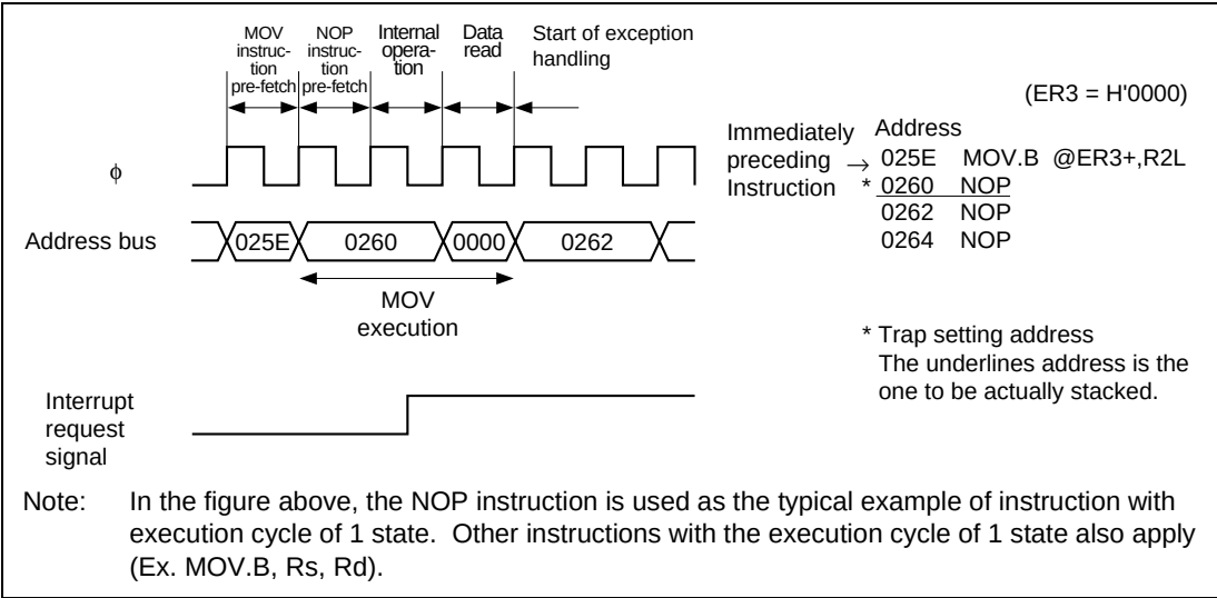
Figure 25.2 Basic Operations (1)
