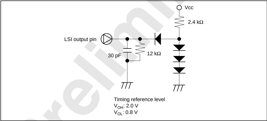
Figure 30.8 Output Load Conditions
