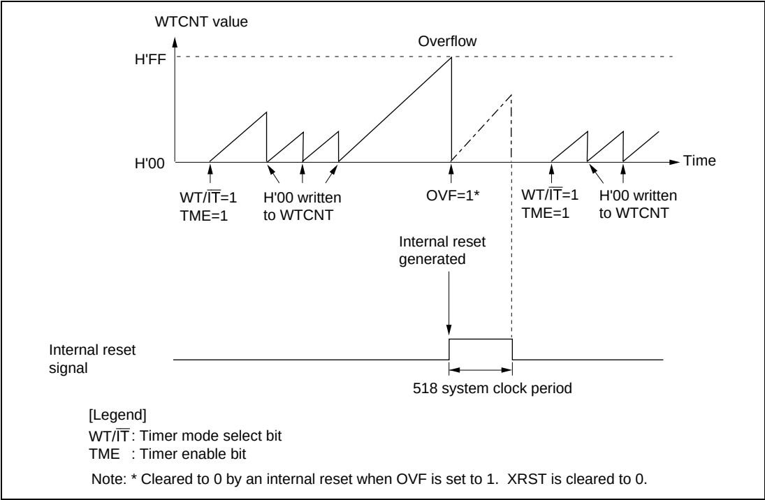
Figure 17.3 Operation in Watchdog Timer Mode (when Reset)
