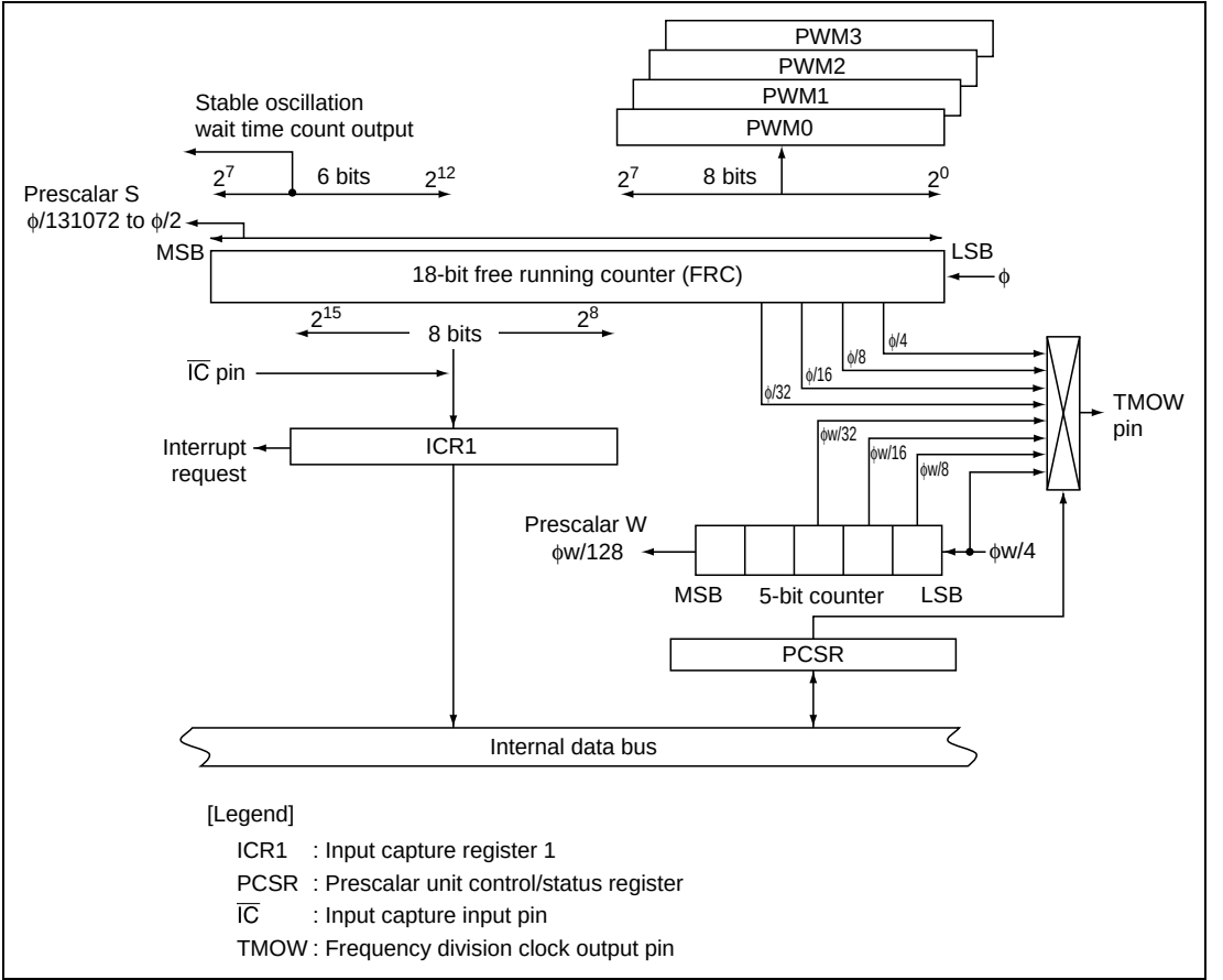
Figure 21.1 Block Diagram of Prescaler Unit
