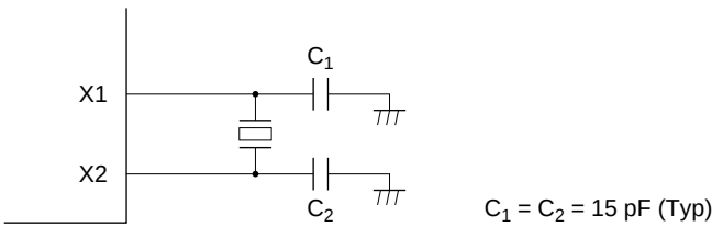
Figure 9.8 Connecting a 32.768 kHz Crystal Resonator (Example)
