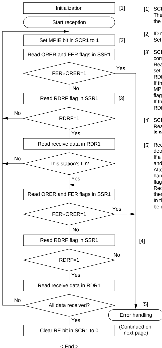
Figure 22.13 Sample Multiprocessor Serial Reception Flowchart (1)
