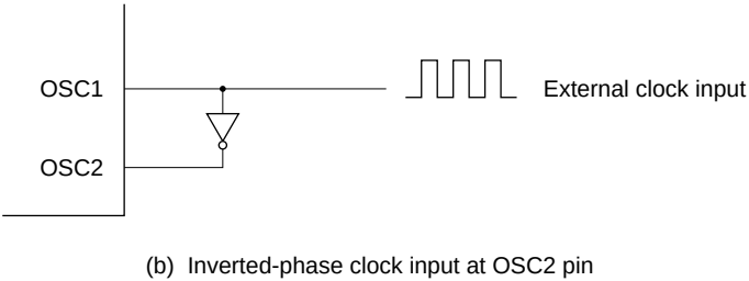
Figure 9.5 External Clock Input (Examples)
