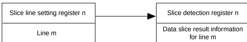
Figure 28.5 Relationship between Slice Line Setting Register and Slice Detection Register
