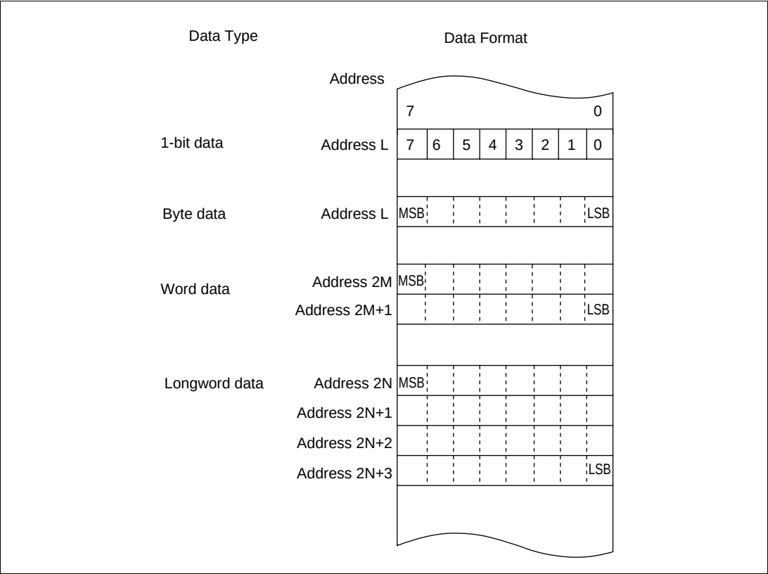
Figure 2.12 Memory Data Formats
