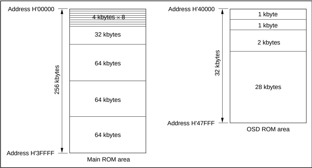
Figure 7.6 Flash Memory Block Configuration
