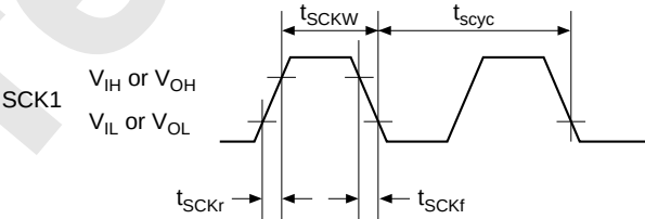
Figure 30.6 SCK1 Clock Timing
