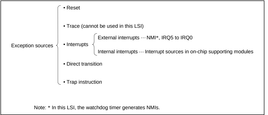
Figure 5.1 Exception Sources
