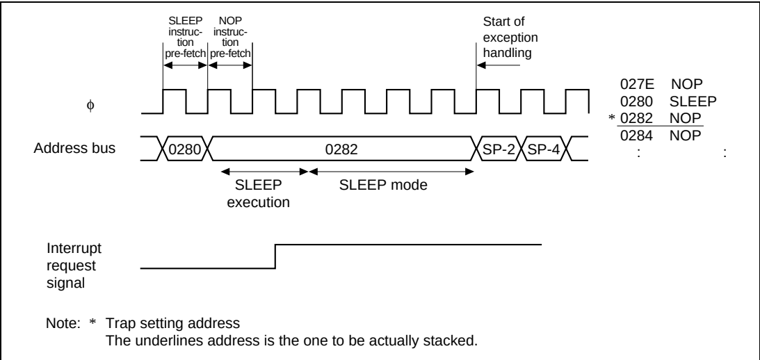
Figure 25.18 SLEEP Instruction (3)
