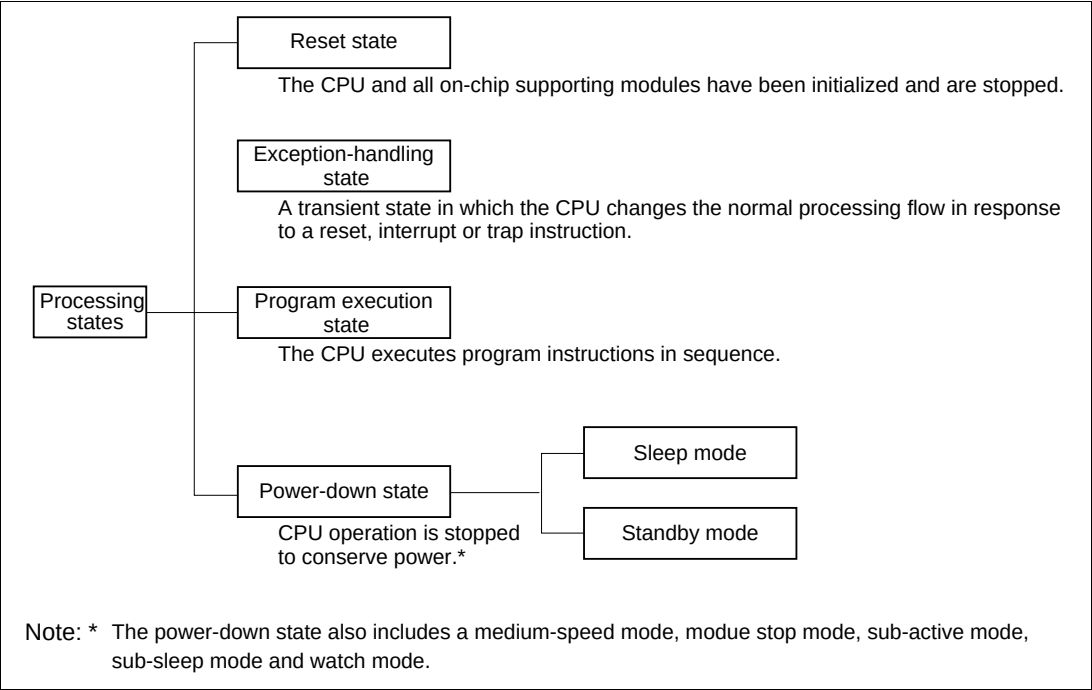
Figure 2.15 Processing States
