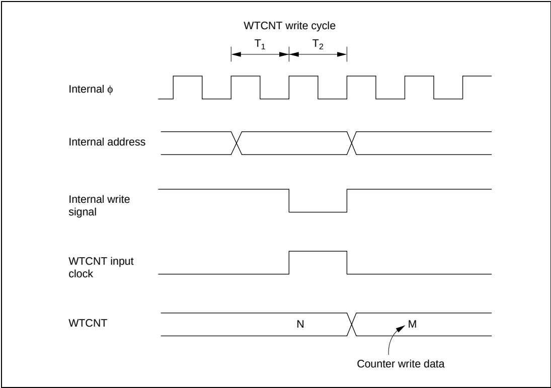
Figure 17.6 Contention between WTCNT Write and Increment
