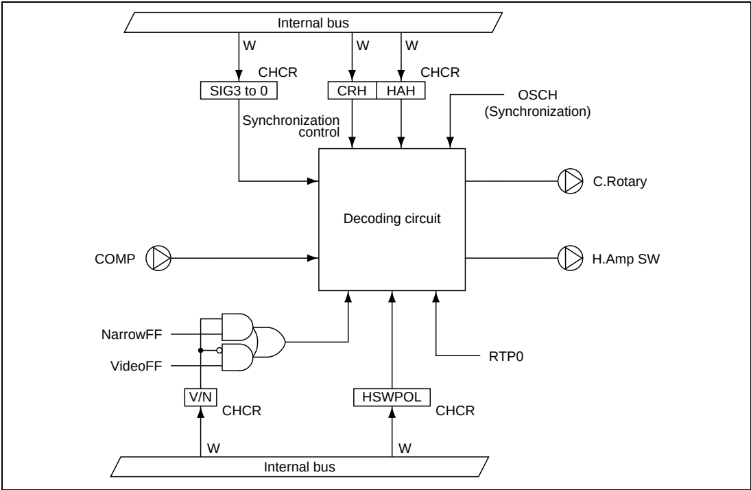
Figure 26.26 High-Speed Switching Circuit for Four-Head Special Playback
