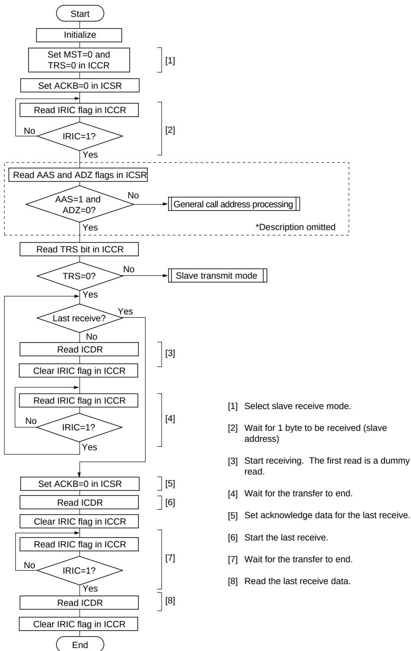
Figure 23.16 Flowchart for Slave Transmit Mode (Example)
