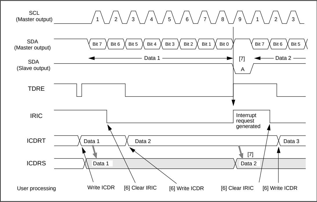
Figure 23.7 Example of Continuous Transmission Timing in Master Transmit Mode (MLS = WAIT = 0)
