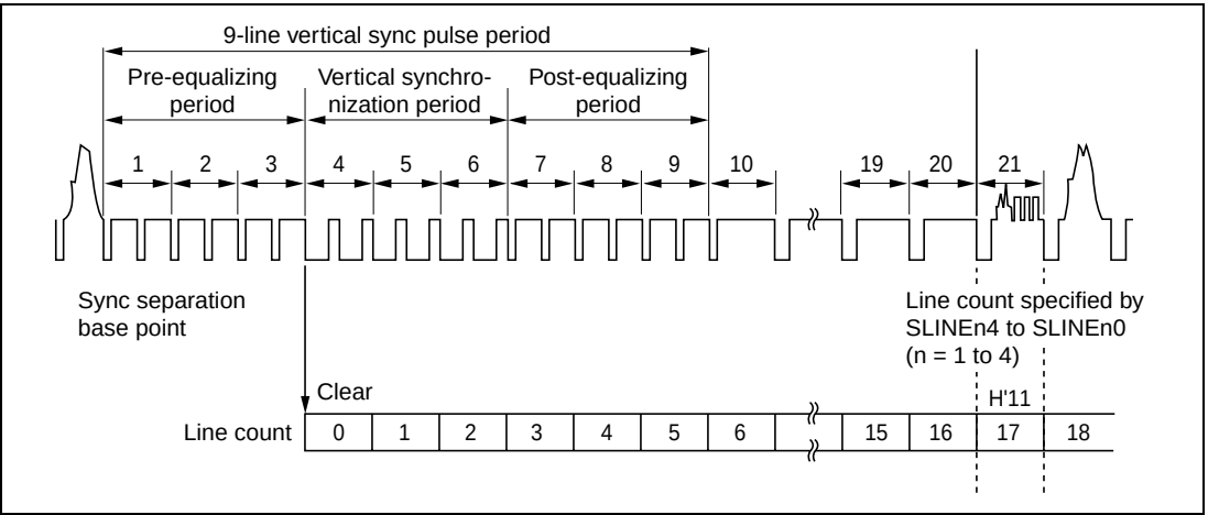
Figure 28.4 Line Count
