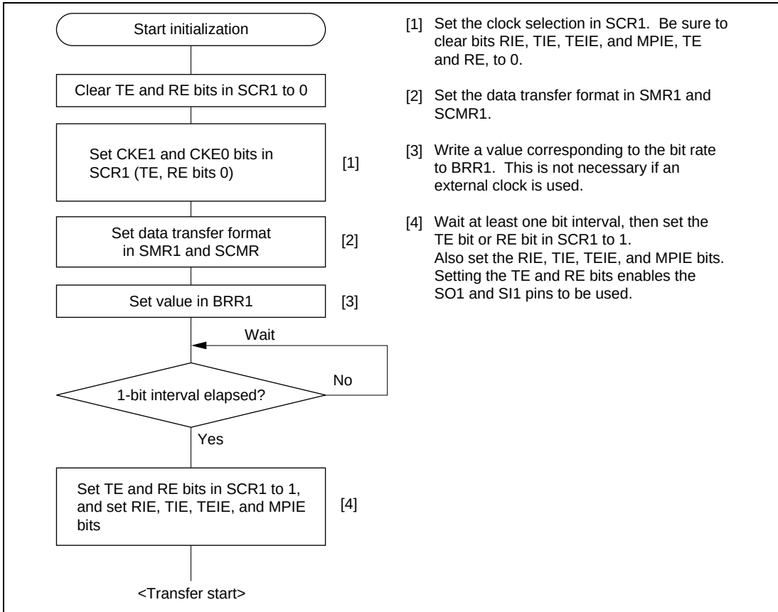
Figure 22.17 Sample SCI Initialization Flowchart
