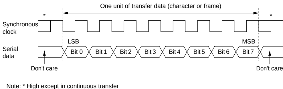
Figure 22.16 Data Format in Synchronous Communication
