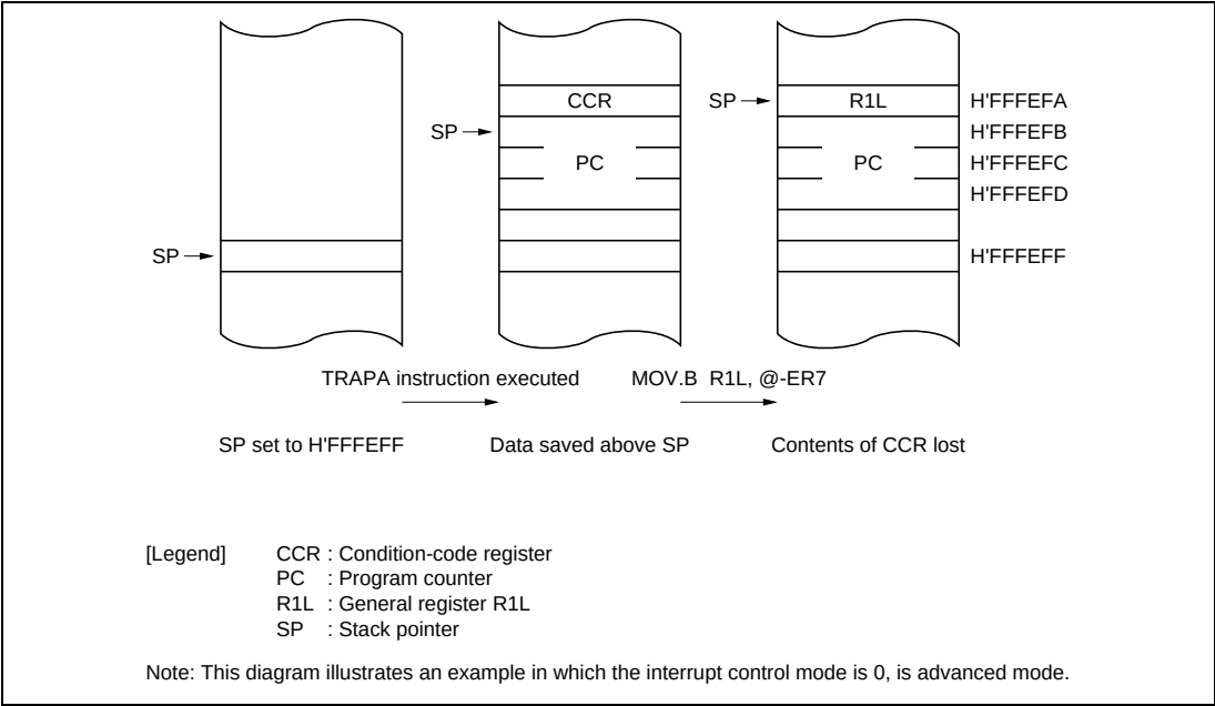
Figure 5.6 Operation when SP Value is Odd
