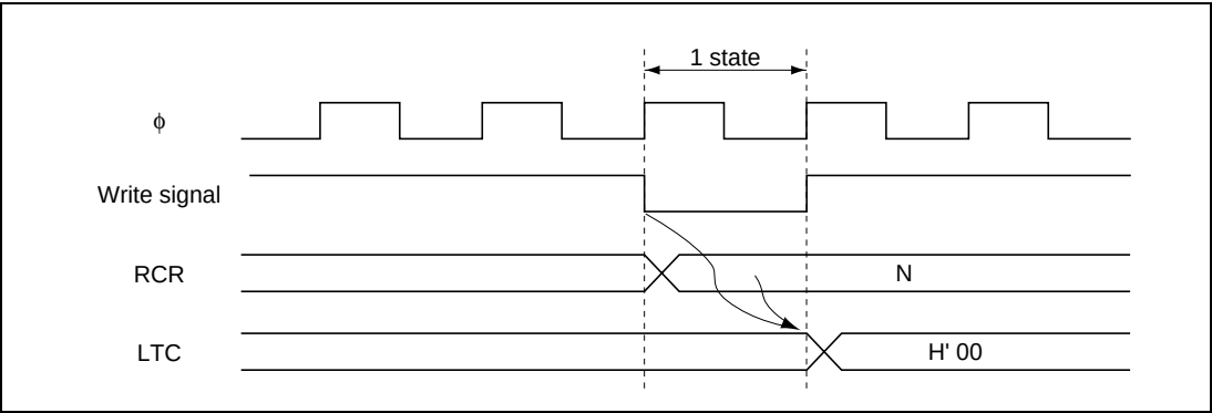
Figure 14.2 RCR Writing and LTC Clearing Timing Chart
