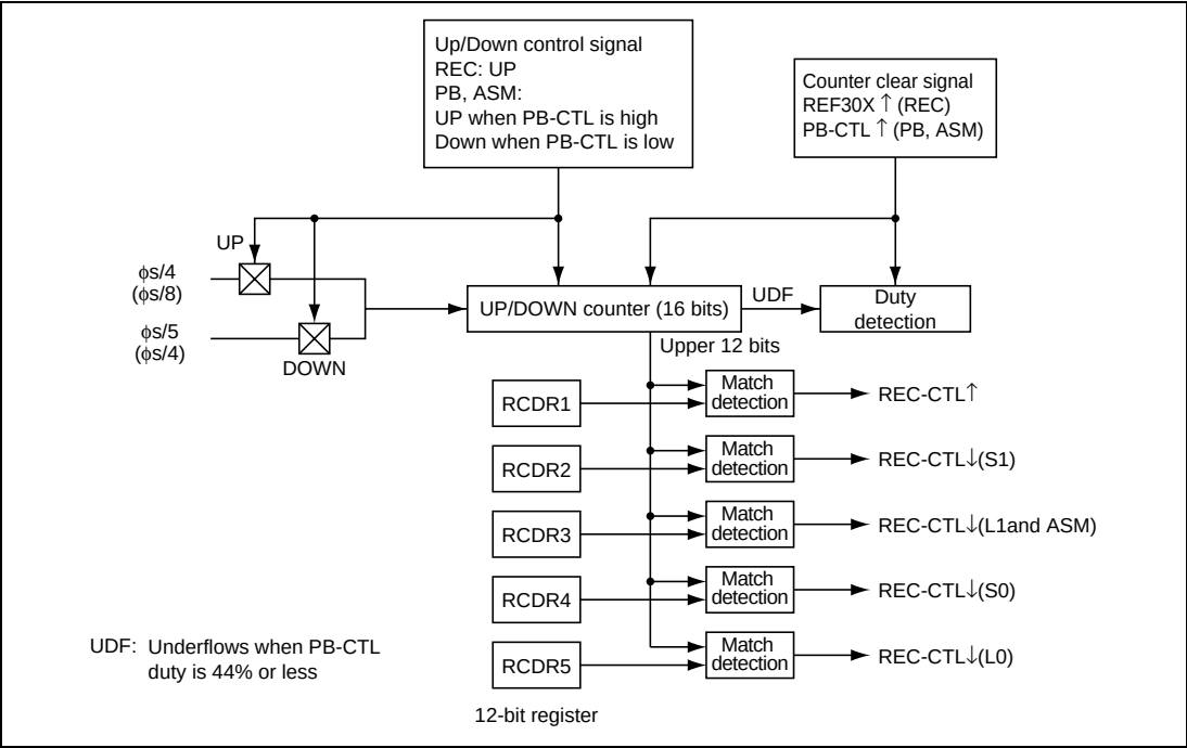
Figure 26.49 CTL Discrimination/Record Circuit
