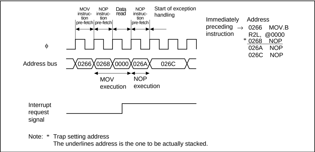
Figure 25.3 Basic Operations (2)
