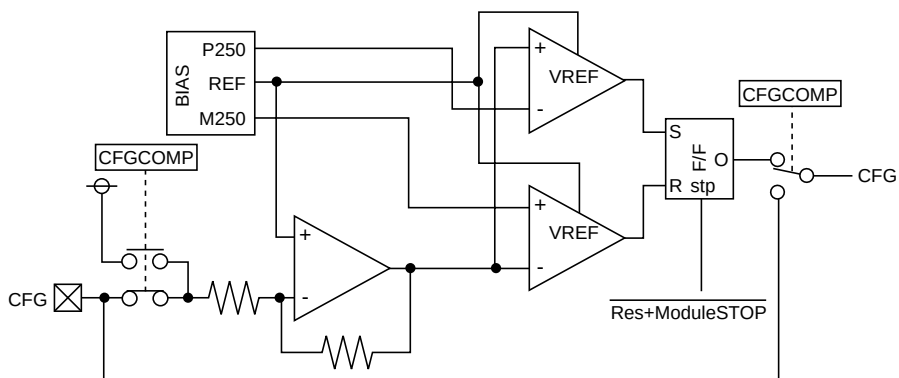
Figure 26.3 CFG Input Circuit
