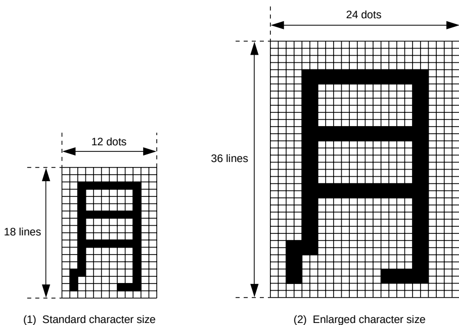
Figure 29.3 Enlarged Character Example
