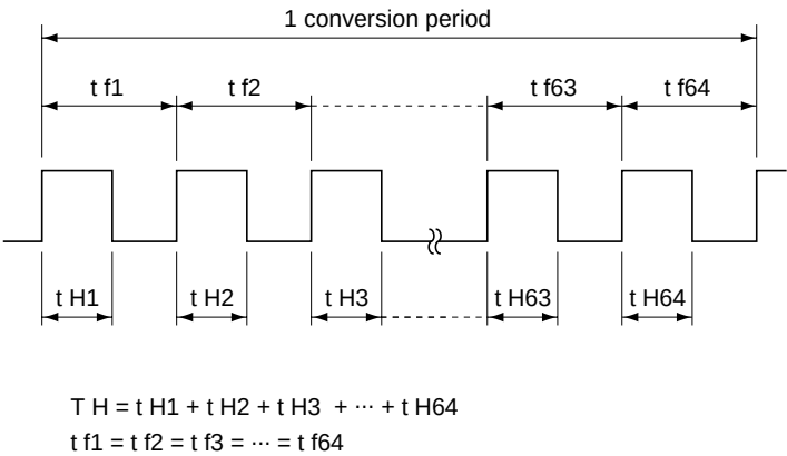
Figure 20.2 Waveform Output by 14-Bit PWM
