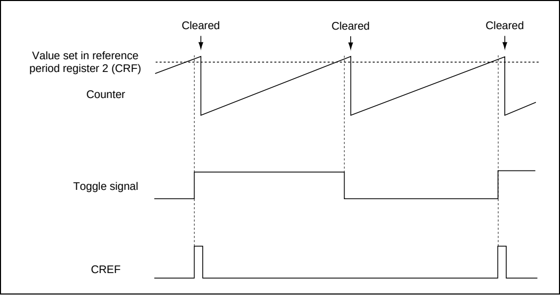
Figure 26.13 Generation of CREF Signal
