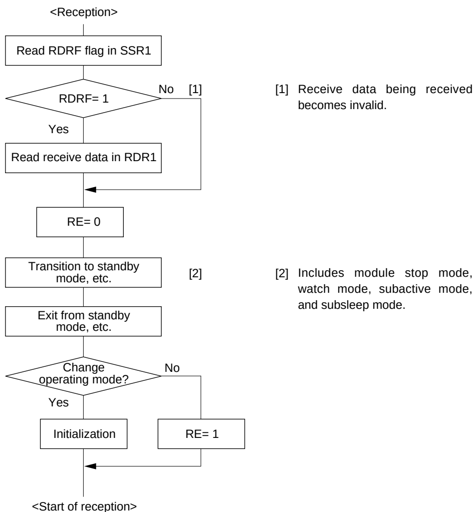
Figure 22.27 Sample Flowchart for Mode Transition during Reception
