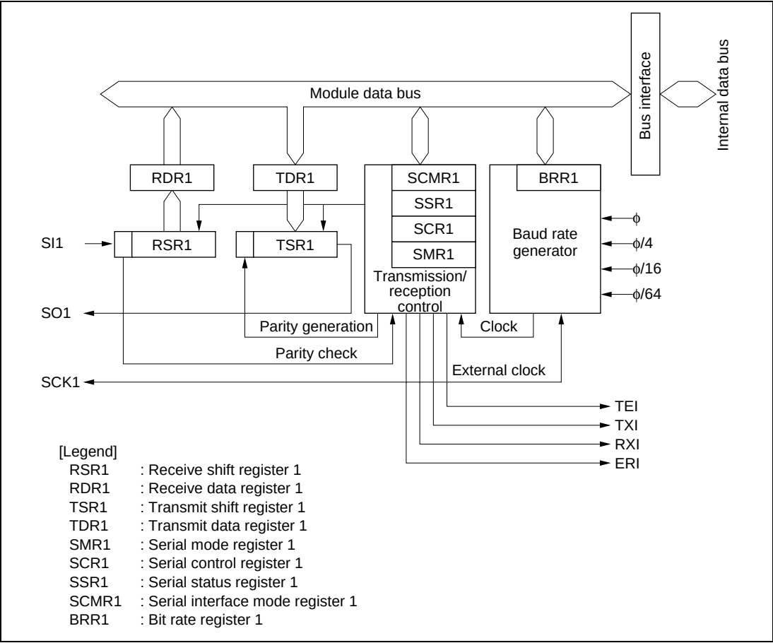
Figure 22.1 Block Diagram of SCI
