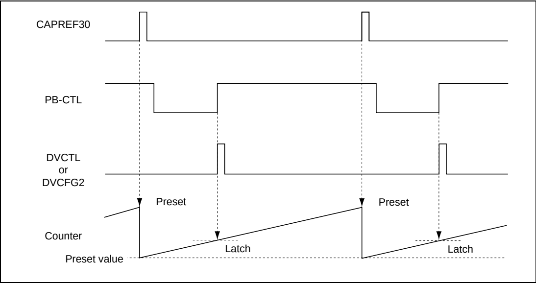
Figure 26.35 Capstan Phase Control in Playback Mode
