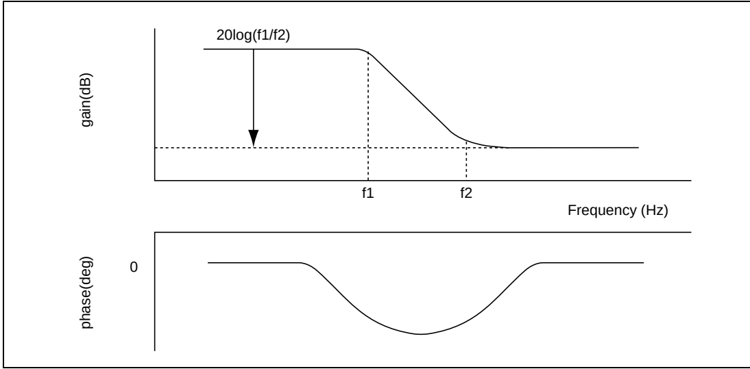
Figure 26.41 Frequency Characteristics of the Lag-Lead Filter
