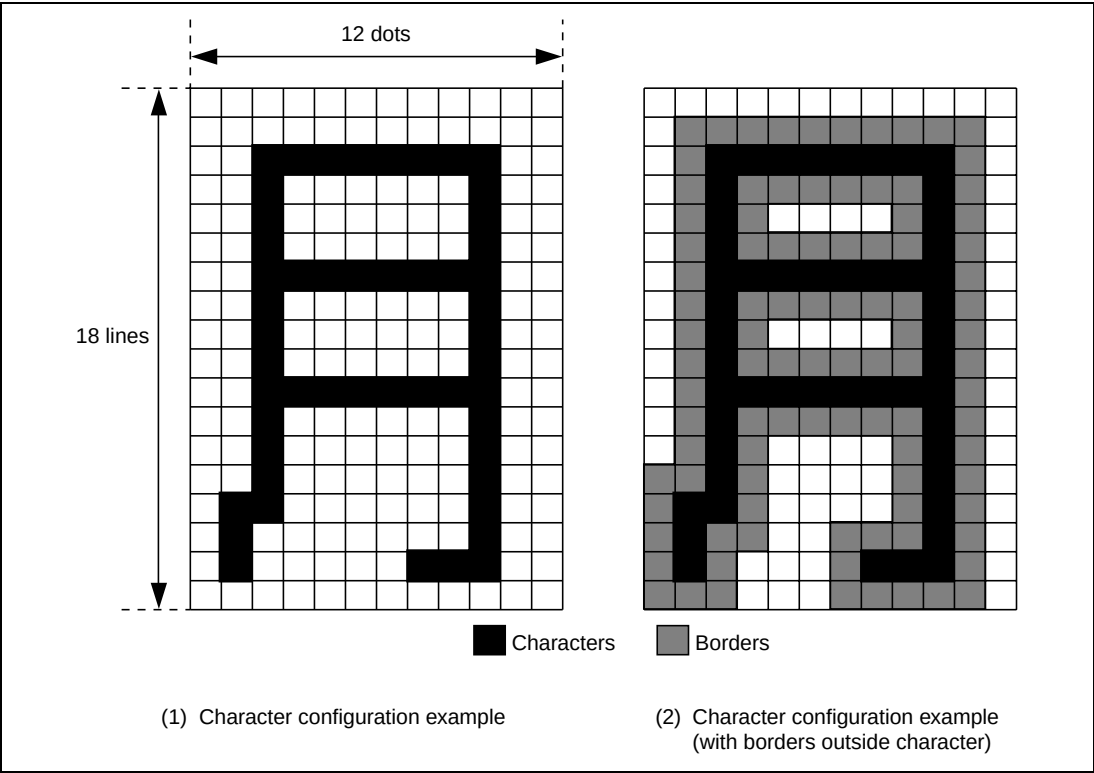
Figure 29.2 Character Configuration Examples
