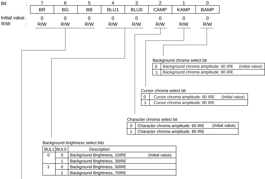
Background color specification (Background Colors in Text Display Mode)
